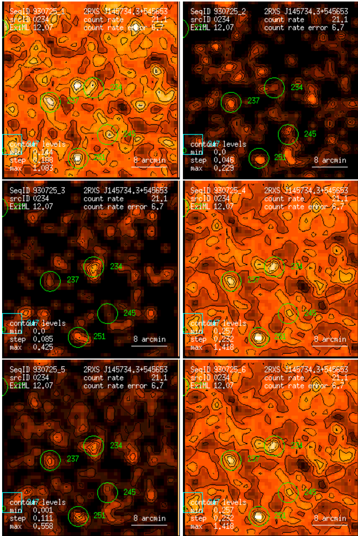
Figure 234: RASS 930725: detection 0234: band rate images, Gaussian filter: (1) PSPC channels 11 – 41, (2) 52 – 90, (3) 91 – 201, (4) 11 – 235, (5) 52 – 201, (6) 11 – 201. Broad band rates in counts/ks. Band rate contour levels in counts/ks/arcmin 2 .
