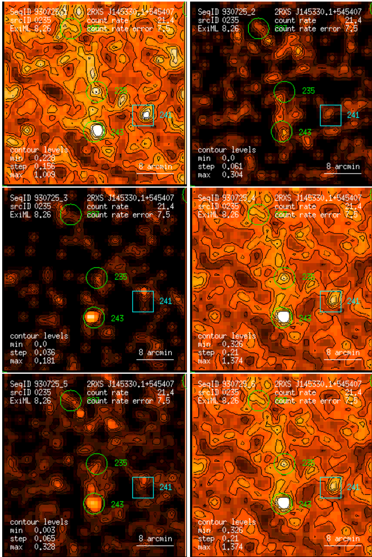
Figure 235: RASS 930725: detection 0235: band rate images, Gaussian filter: (1) PSPC channels 11 – 41, (2) 52 – 90, (3) 91 – 201, (4) 11 – 235, (5) 52 – 201, (6) 11 – 201. Broad band rates in counts/ks. Band rate contour levels in counts/ks/arcmin 2 .
