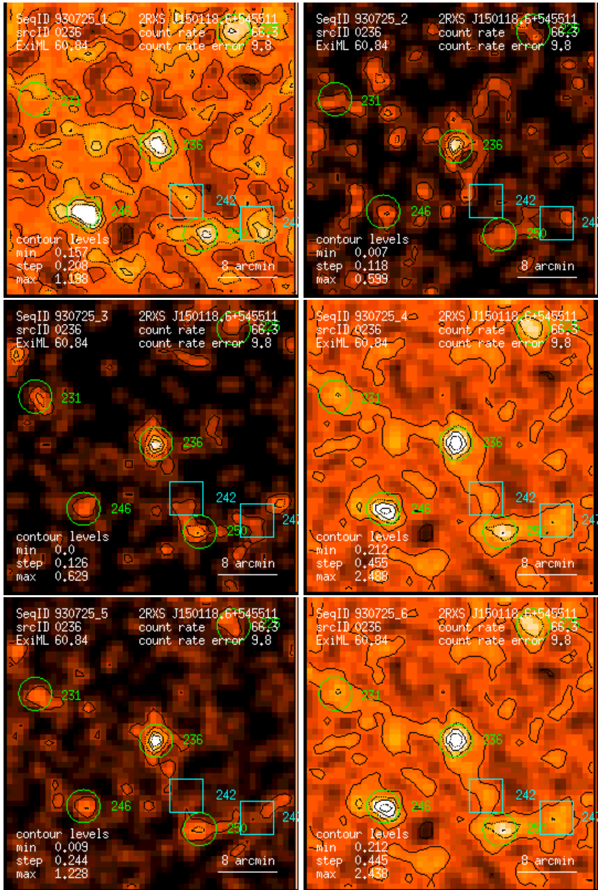
Figure 236: RASS 930725: detection 0236: band rate images, Gaussian filter: (1) PSPC channels 11 – 41, (2) 52 – 90, (3) 91 – 201, (4) 11 – 235, (5) 52 – 201, (6) 11 – 201. Broad band rates in counts/ks. Band rate contour levels in counts/ks/arcmin 2 .
