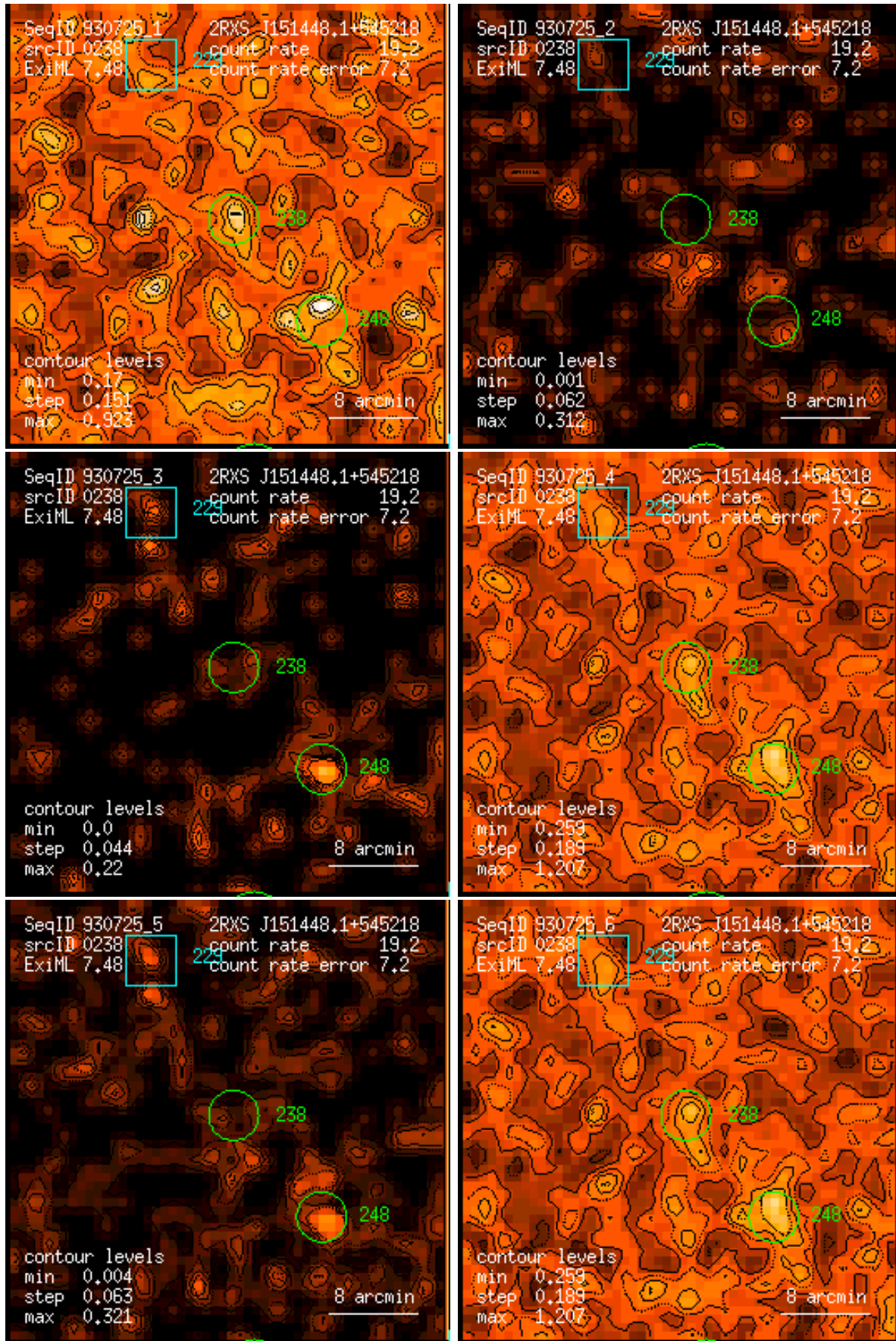
Figure 238: RASS 930725: detection 0238: band rate images, Gaussian filter: (1) PSPC channels 11 – 41, (2) 52 – 90, (3) 91 – 201, (4) 11 – 235, (5) 52 – 201, (6) 11 – 201. Broad band rates in counts/ks. Band rate contour levels in counts/ks/arcmin 2 .
