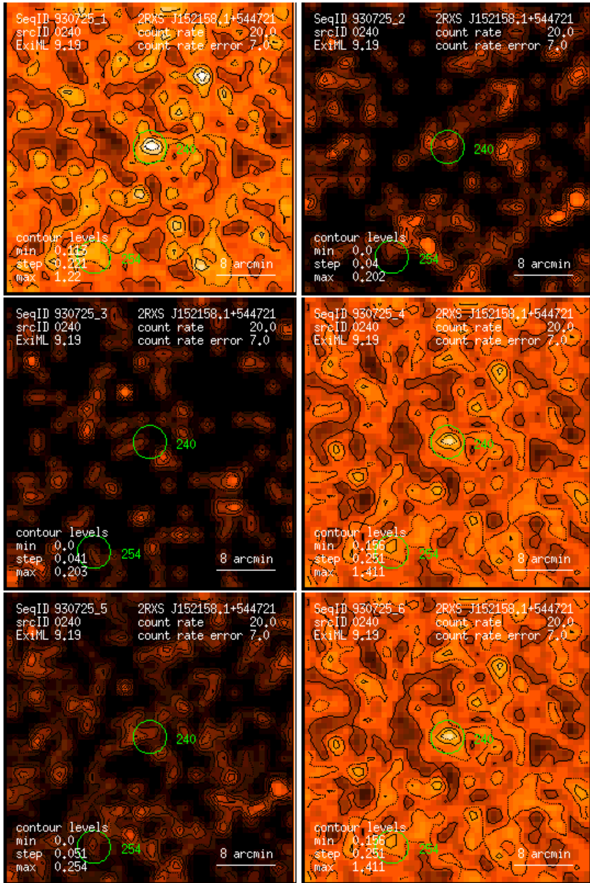
Figure 240: RASS 930725: detection 0240: band rate images, Gaussian filter: (1) PSPC channels 11 – 41, (2) 52 – 90, (3) 91 – 201, (4) 11 – 235, (5) 52 – 201, (6) 11 – 201. Broad band rates in counts/ks. Band rate contour levels in counts/ks/arcmin 2 .
