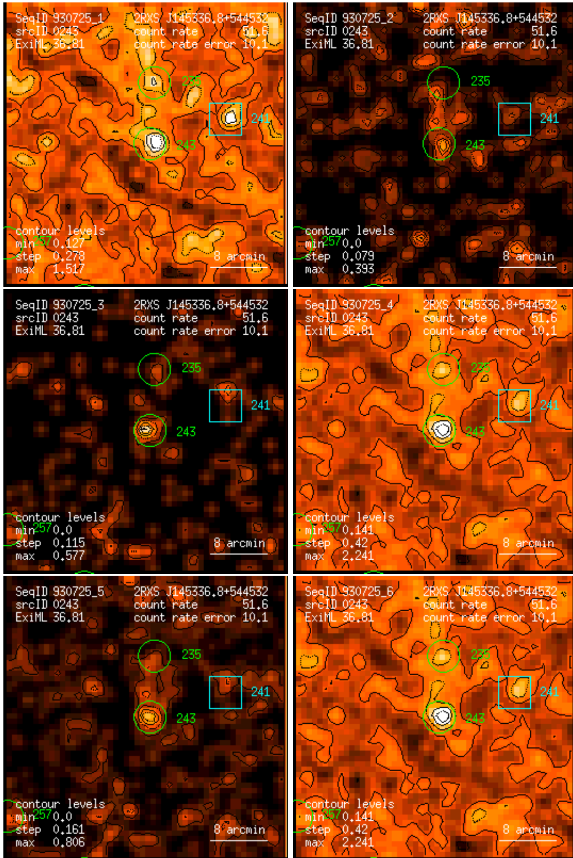
Figure 243: RASS 930725: detection 0243: band rate images, Gaussian filter: (1) PSPC channels 11 – 41, (2) 52 – 90, (3) 91 – 201, (4) 11 – 235, (5) 52 – 201, (6) 11 – 201. Broad band rates in counts/ks. Band rate contour levels in counts/ks/arcmin 2 .
