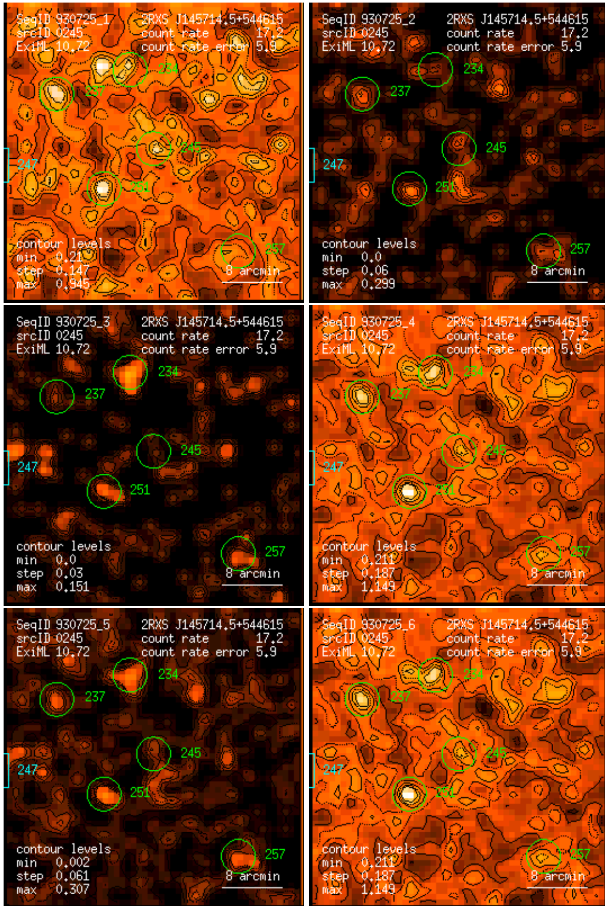
Figure 245: RASS 930725: detection 0245: band rate images, Gaussian filter: (1) PSPC channels 11 – 41, (2) 52 – 90, (3) 91 – 201, (4) 11 – 235, (5) 52 – 201, (6) 11 – 201. Broad band rates in counts/ks. Band rate contour levels in counts/ks/arcmin 2 .
