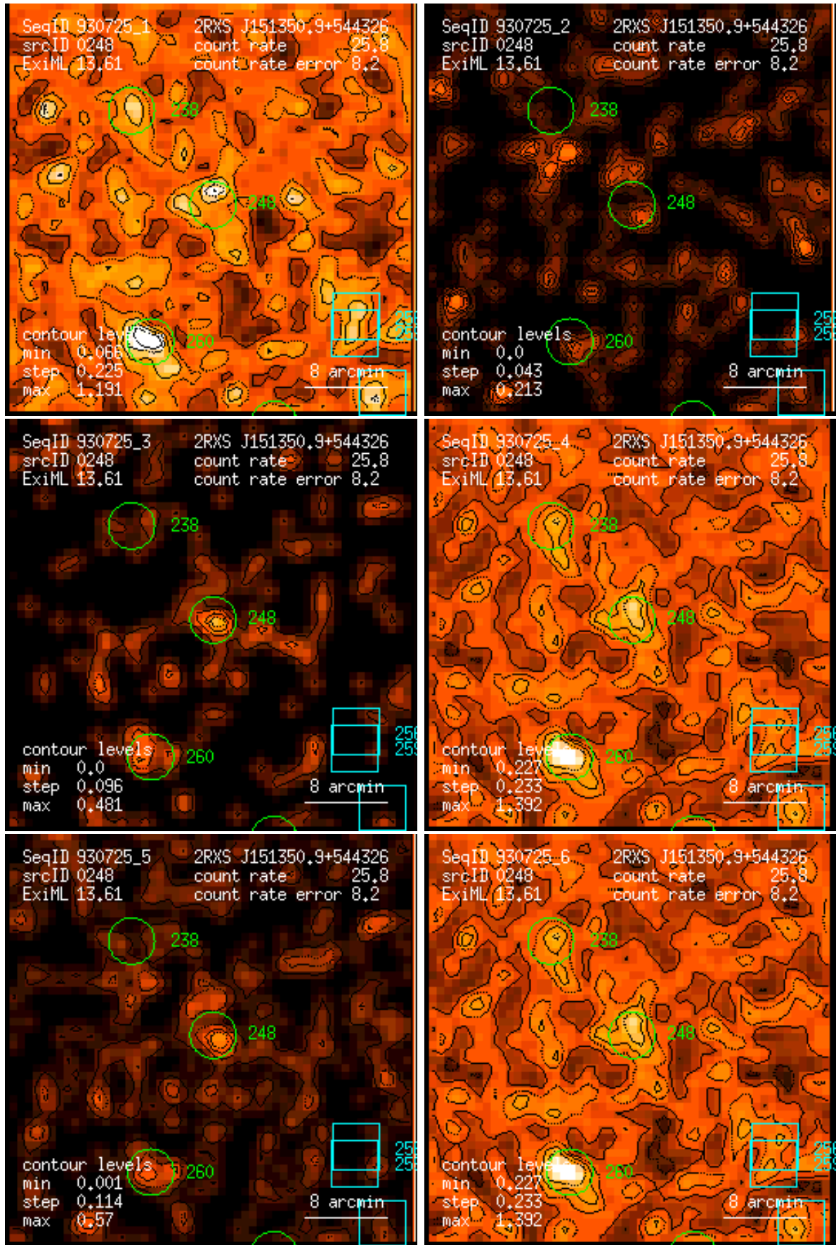
Figure 248: RASS 930725: detection 0248: band rate images, Gaussian filter: (1) PSPC channels 11 – 41, (2) 52 – 90, (3) 91 – 201, (4) 11 – 235, (5) 52 – 201, (6) 11 – 201. Broad band rates in counts/ks. Band rate contour levels in counts/ks/arcmin 2 .
