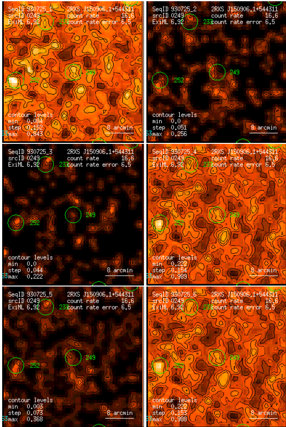
Figure 249: RASS 930725: detection 0249: band rate images, Gaussian filter: (1) PSPC channels 11 – 41, (2) 52 – 90, (3) 91 – 201, (4) 11 – 235, (5) 52 – 201, (6) 11 – 201. Broad band rates in counts/ks. Band rate contour levels in counts/ks/arcmin 2 .
