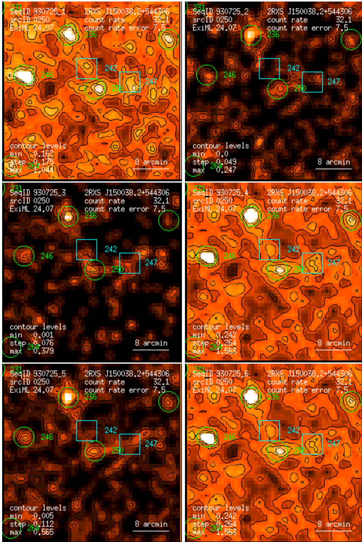
Figure 250: RASS 930725: detection 0250: band rate images, Gaussian filter: (1) PSPC channels 11 – 41, (2) 52 – 90, (3) 91 – 201, (4) 11 – 235, (5) 52 – 201, (6) 11 – 201. Broad band rates in counts/ks. Band rate contour levels in counts/ks/arcmin 2 .
