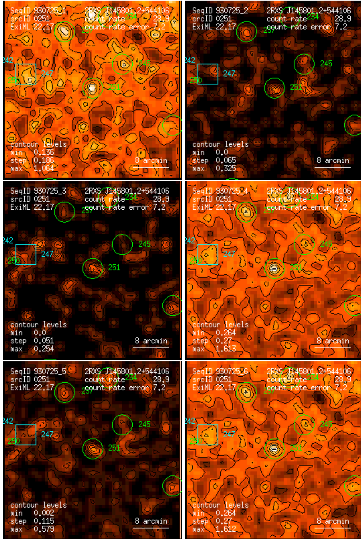
Figure 251: RASS 930725: detection 0251: band rate images, Gaussian filter: (1) PSPC channels 11 – 41, (2) 52 – 90, (3) 91 – 201, (4) 11 – 235, (5) 52 – 201, (6) 11 – 201. Broad band rates in counts/ks. Band rate contour levels in counts/ks/arcmin 2 .
