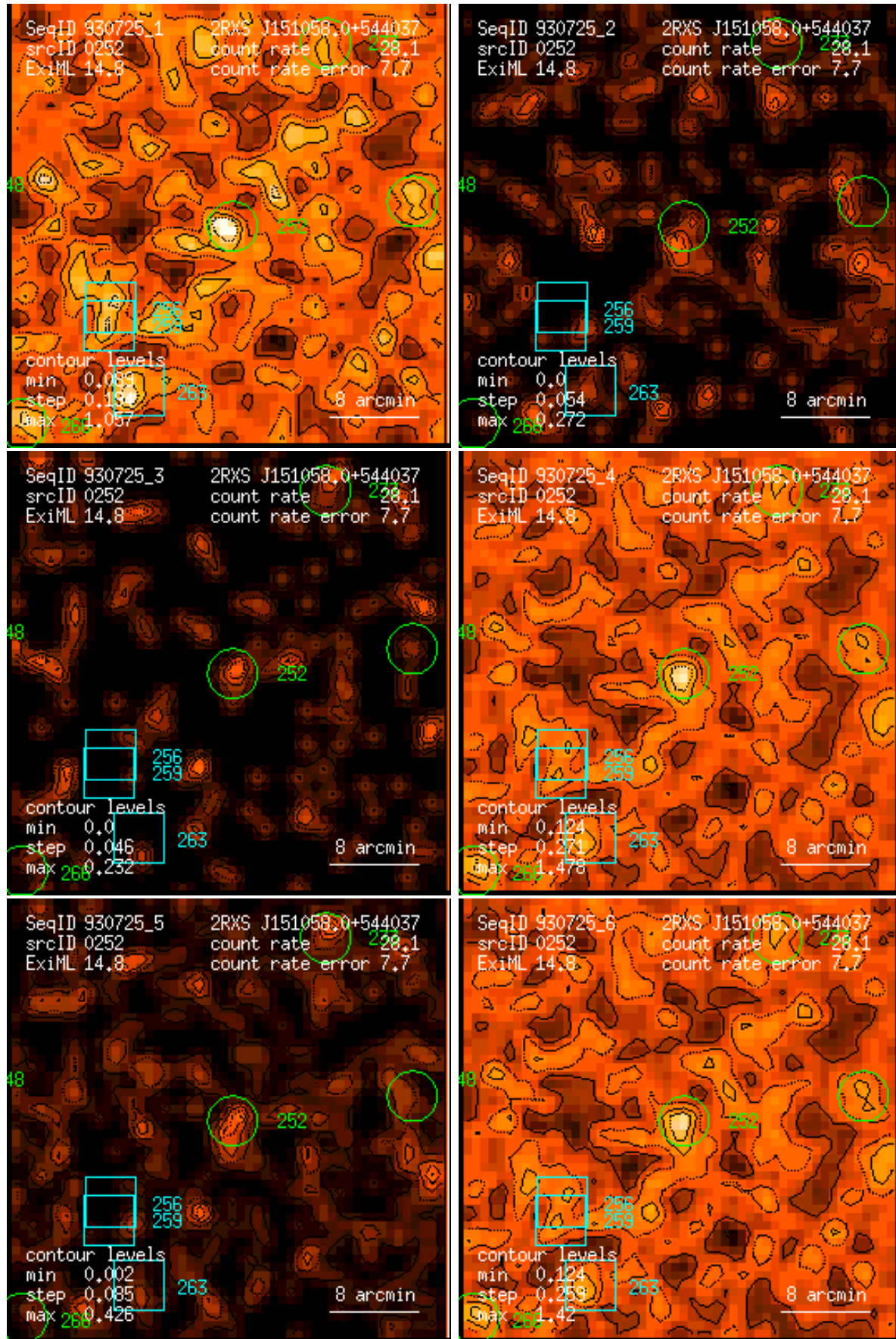
Figure 252: RASS 930725: detection 0252: band rate images, Gaussian filter: (1) PSPC channels 11 – 41, (2) 52 – 90, (3) 91 – 201, (4) 11 – 235, (5) 52 – 201, (6) 11 – 201. Broad band rates in counts/ks. Band rate contour levels in counts/ks/arcmin 2 .
