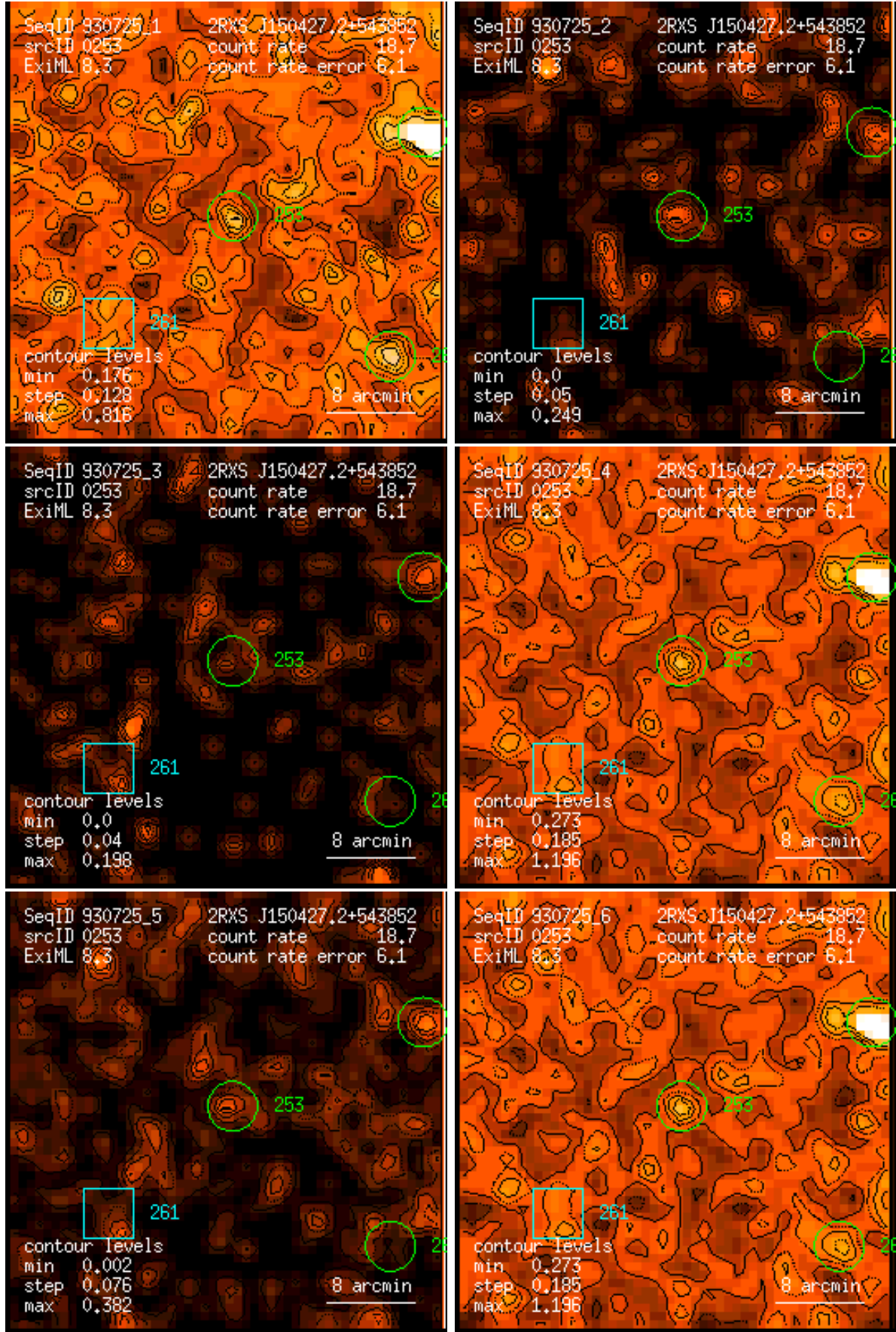
Figure 253: RASS 930725: detection 0253: band rate images, Gaussian filter: (1) PSPC channels 11 – 41, (2) 52 – 90, (3) 91 – 201, (4) 11 – 235, (5) 52 – 201, (6) 11 – 201. Broad band rates in counts/ks. Band rate contour levels in counts/ks/arcmin 2 .
