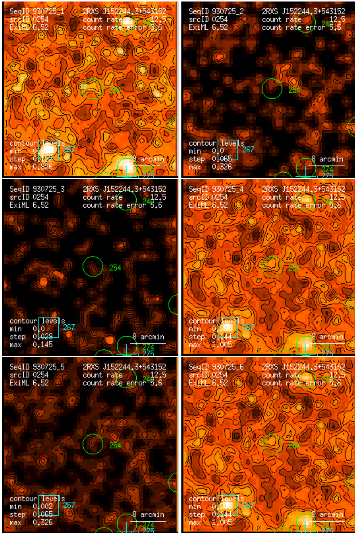
Figure 254: RASS 930725: detection 0254: band rate images, Gaussian filter: (1) PSPC channels 11 – 41, (2) 52 – 90, (3) 91 – 201, (4) 11 – 235, (5) 52 – 201, (6) 11 – 201. Broad band rates in counts/ks. Band rate contour levels in counts/ks/arcmin 2 .
