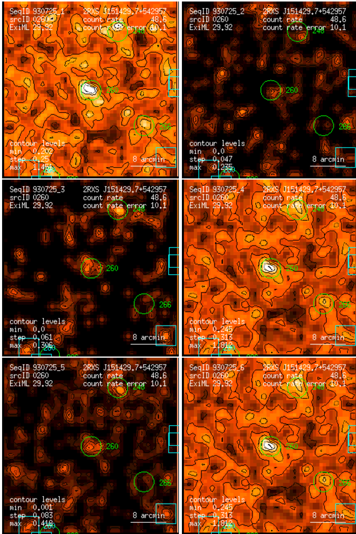
Figure 260: RASS 930725: detection 0260: band rate images, Gaussian filter: (1) PSPC channels 11 – 41, (2) 52 – 90, (3) 91 – 201, (4) 11 – 235, (5) 52 – 201, (6) 11 – 201. Broad band rates in counts/ks. Band rate contour levels in counts/ks/arcmin 2 .
