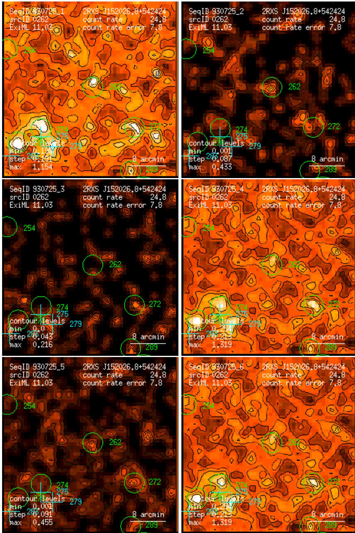
Figure 262: RASS 930725: detection 0262: band rate images, Gaussian filter: (1) PSPPC channels 11 – 41, (2) 52 – 90, (3) 91 – 201, (4) 11 – 235, (5) 52 – 201, (6) 11 – 201. Broad band rates in counts/ks. Band rate contour levels in counts/ks/arcmin 2 .
