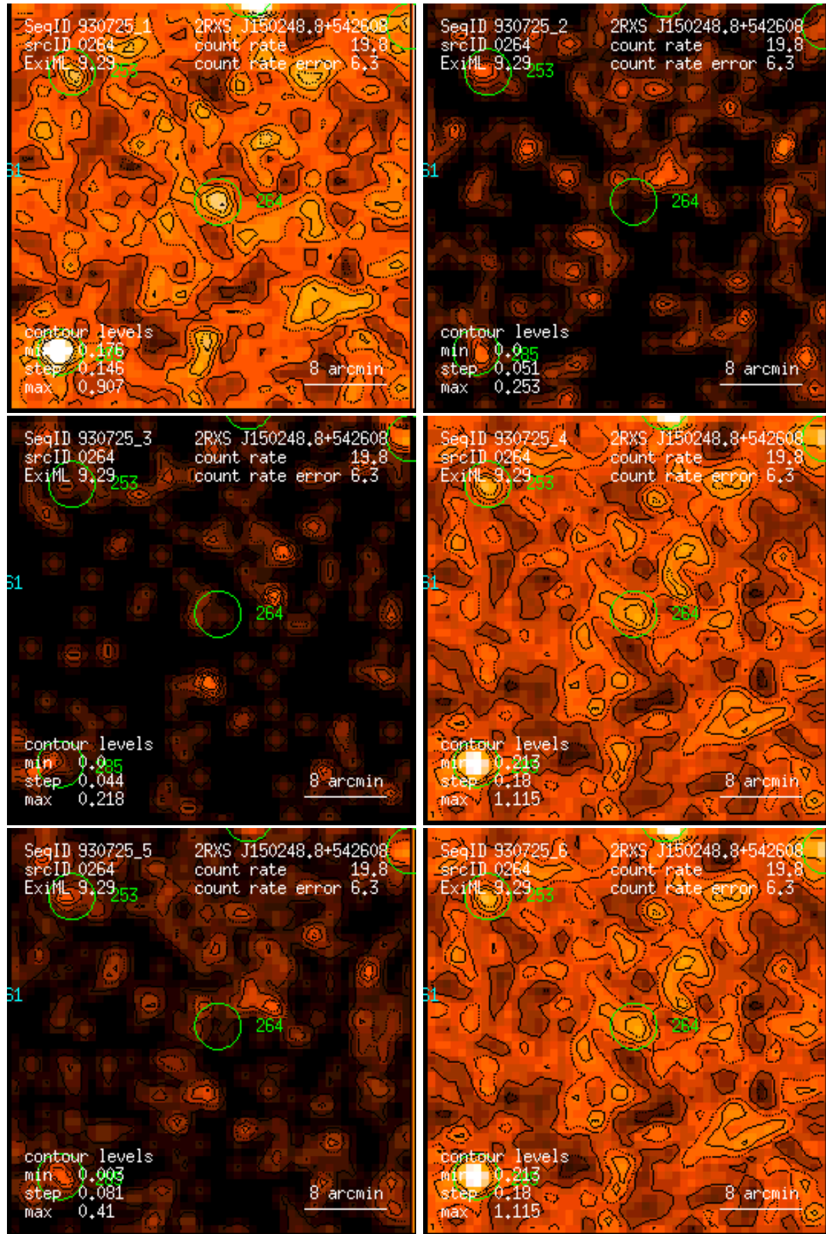
Figure 264: RASS 930725: detection 0264: band rate images, Gaussian filter: (1) PSPC channels 11 – 41, (2) 52 – 90, (3) 91 – 201, (4) 11 – 235, (5) 52 – 201, (6) 11 – 201. Broad band rates in counts/ks. Band rate contour levels in counts/ks/arcmin 2 .
