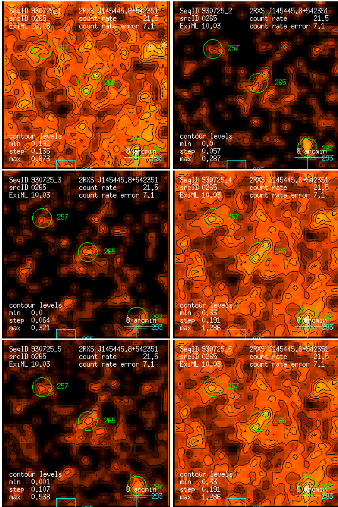
Figure 265: RASS 930725: detection 0265: band rate images, Gaussian filter: (1) PSPC channels 11 – 41, (2) 52 – 90, (3) 91 – 201, (4) 11 – 235, (5) 52 – 201, (6) 11 – 201. Broad band rates in counts/ks. Band rate contour levels in counts/ks/arcmin 2 .
