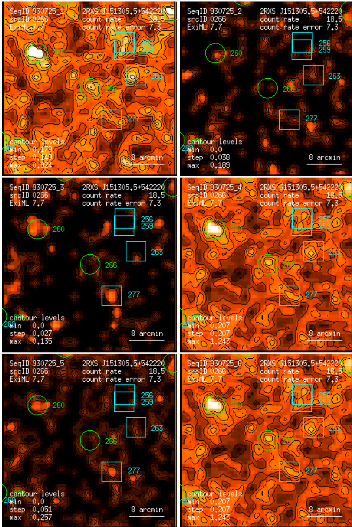
Figure 266: RASS 930725: detection 0266: band rate images, Gaussian filter: (1) PSPC channels 11 – 41, (2) 52 – 90, (3) 91 – 201, (4) 11 – 235, (5) 52 – 201, (6) 11 – 201. Broad band rates in counts/ks. Band rate contour levels in counts/ks/arcmin 2 .
