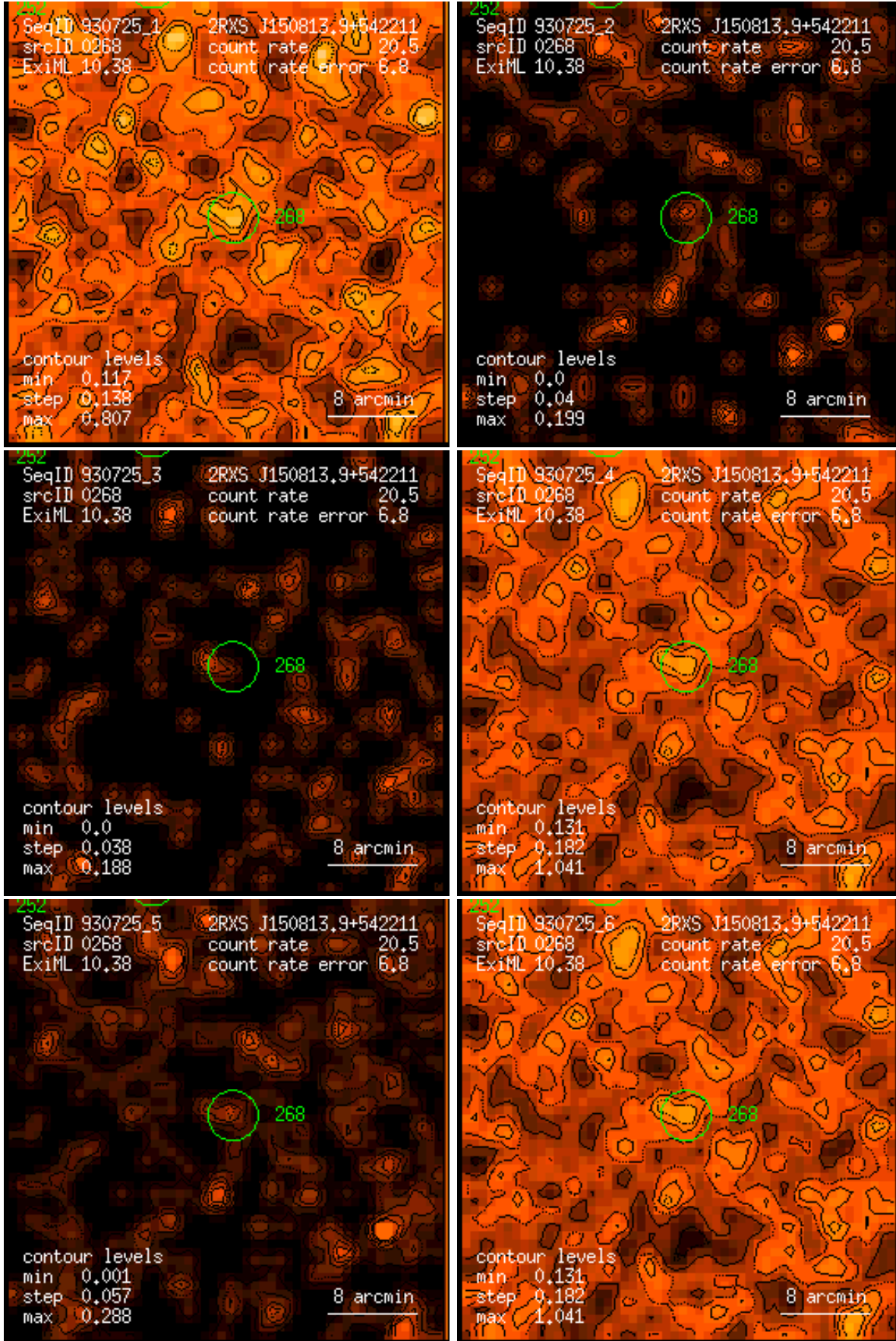
Figure 268: RASS 930725: detection 0268: band rate images, Gaussian filter: (1) PSPC channels 11 – 41, (2) 52 – 90, (3) 91 – 201, (4) 11 – 235, (5) 52 – 201, (6) 11 – 201. Broad band rates in counts/ks. Band rate contour levels in counts/ks/arcmin 2 .
