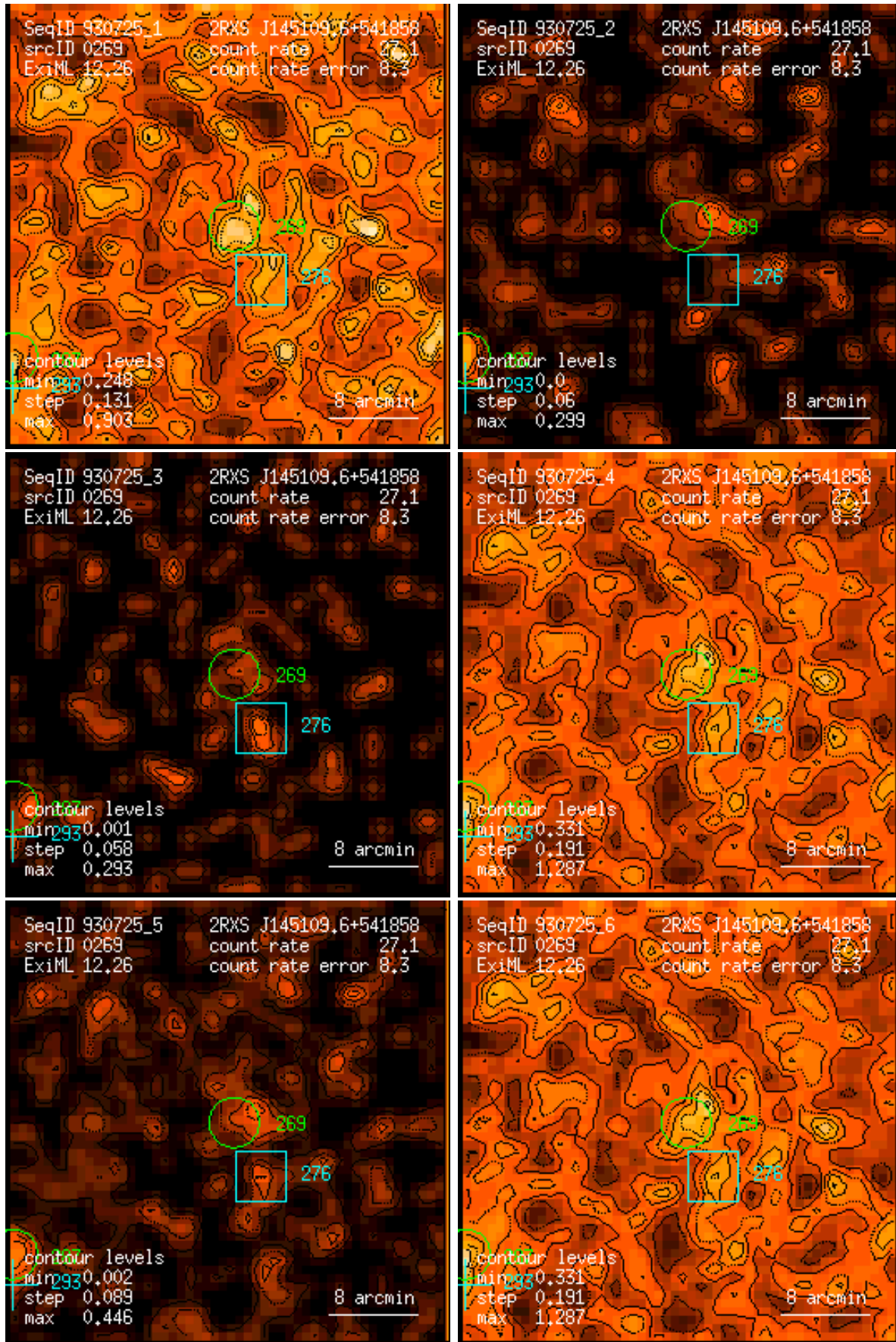
Figure 269: RASS 930725: detection 0269: band rate images, Gaussian filter: (1) PSPC channels 11 – 41, (2) 52 – 90, (3) 91 – 201, (4) 11 – 235, (5) 52 – 201, (6) 11 – 201. Broad band rates in counts/ks. Band rate contour levels in counts/ks/arcmin 2 .
