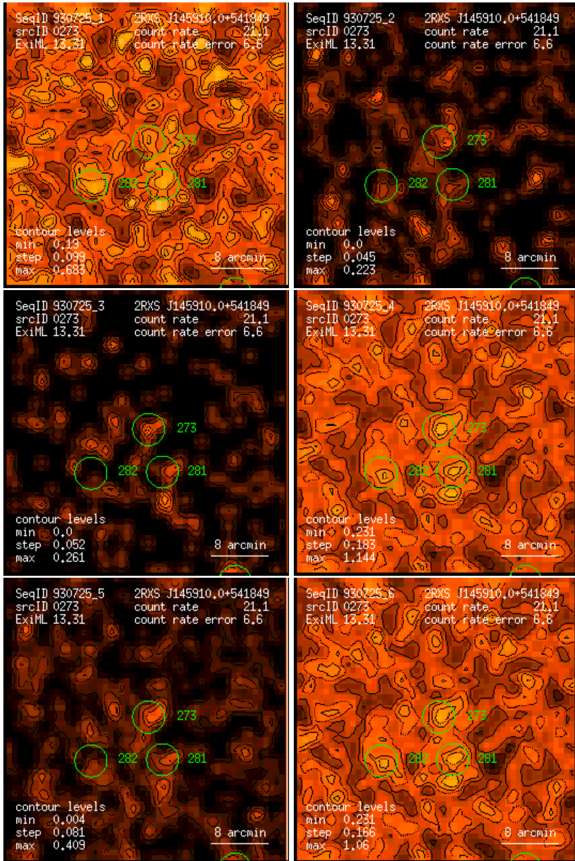
Figure 273: RASS 930725: detection 0273: band rate images, Gaussian filter: (1) PSPC channels 11 – 41, (2) 52 – 90, (3) 91 – 201, (4) 11 – 235, (5) 52 – 201, (6) 11 – 201. Broad band rates in counts/ks. Band rate contour levels in counts/ks/arcmin 2 .
