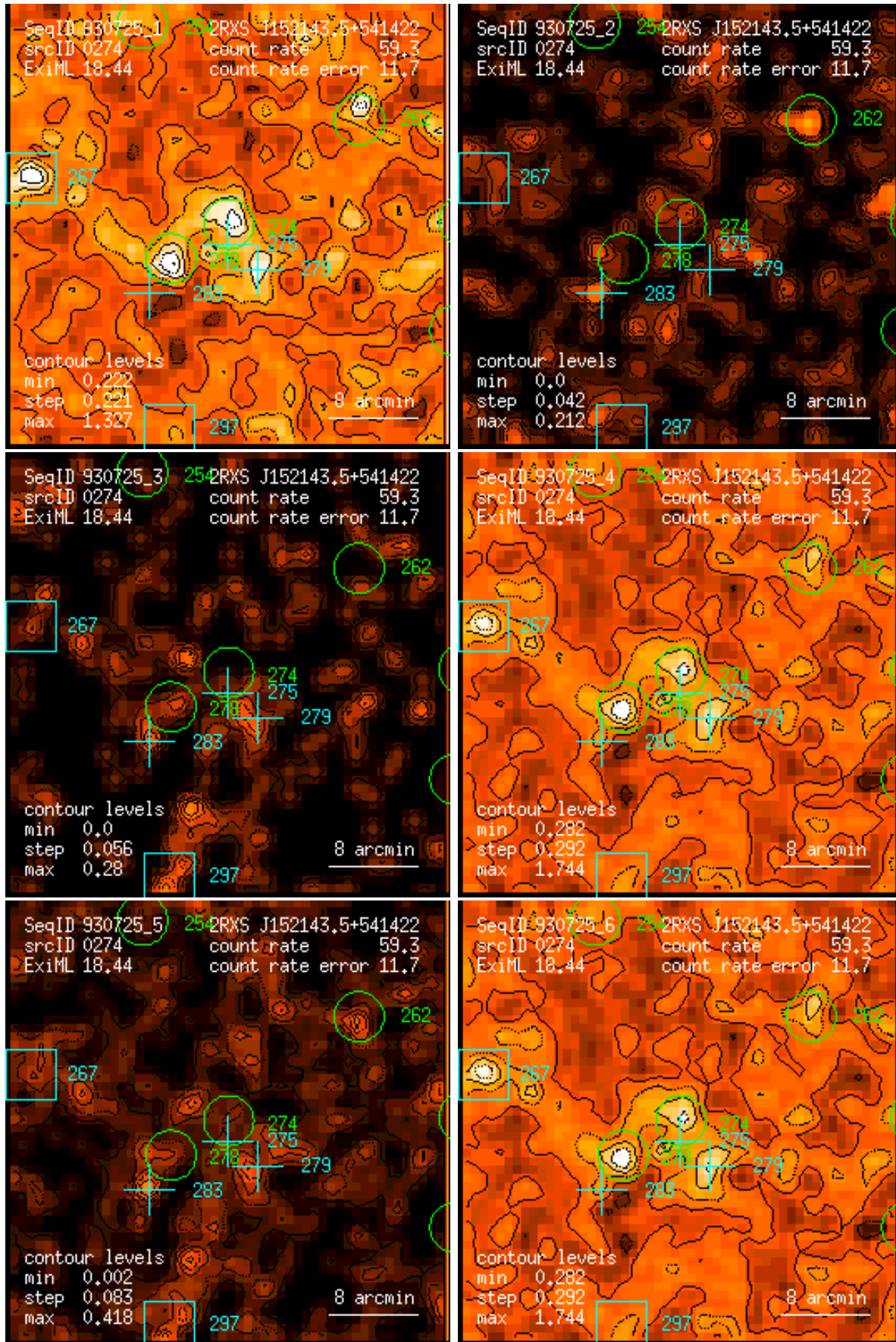
Figure 274: RASS 930725: detection 0274: band rate images, Gaussian filter: (1) PSPC channels 11 – 41, (2) 52 – 90, (3) 91 – 201, (4) 11 – 235, (5) 52 – 201, (6) 11 – 201. Broad band rates in counts/ks. Band rate contour levels in counts/ks/arcmin 2 .
