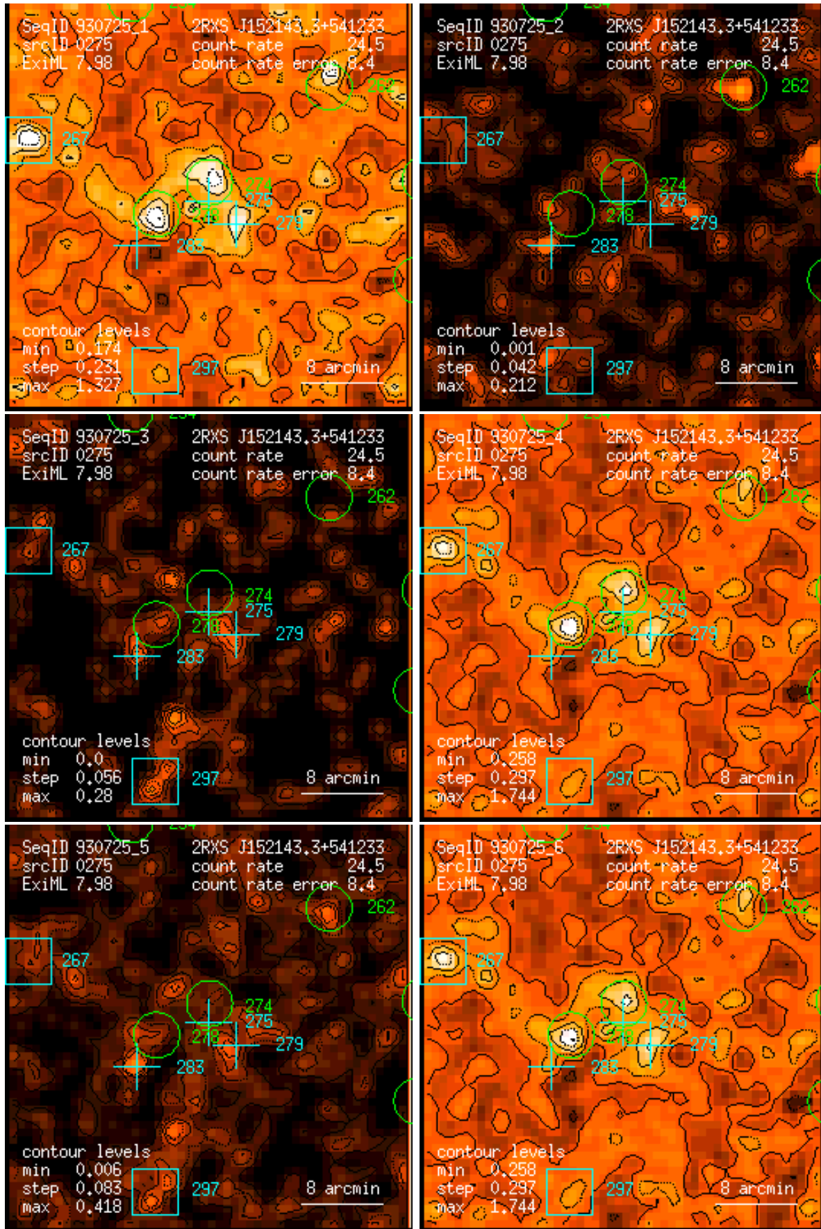
Figure 275: RASS 930725: detection 0275: band rate images, Gaussian filter: (1) PSPC channels 11 – 41, (2) 52 – 90, (3) 91 – 201, (4) 11 – 235, (5) 52 – 201, (6) 11 – 201. Broad band rates in counts/ks. Band rate contour levels in counts/ks/arcmin 2 .
