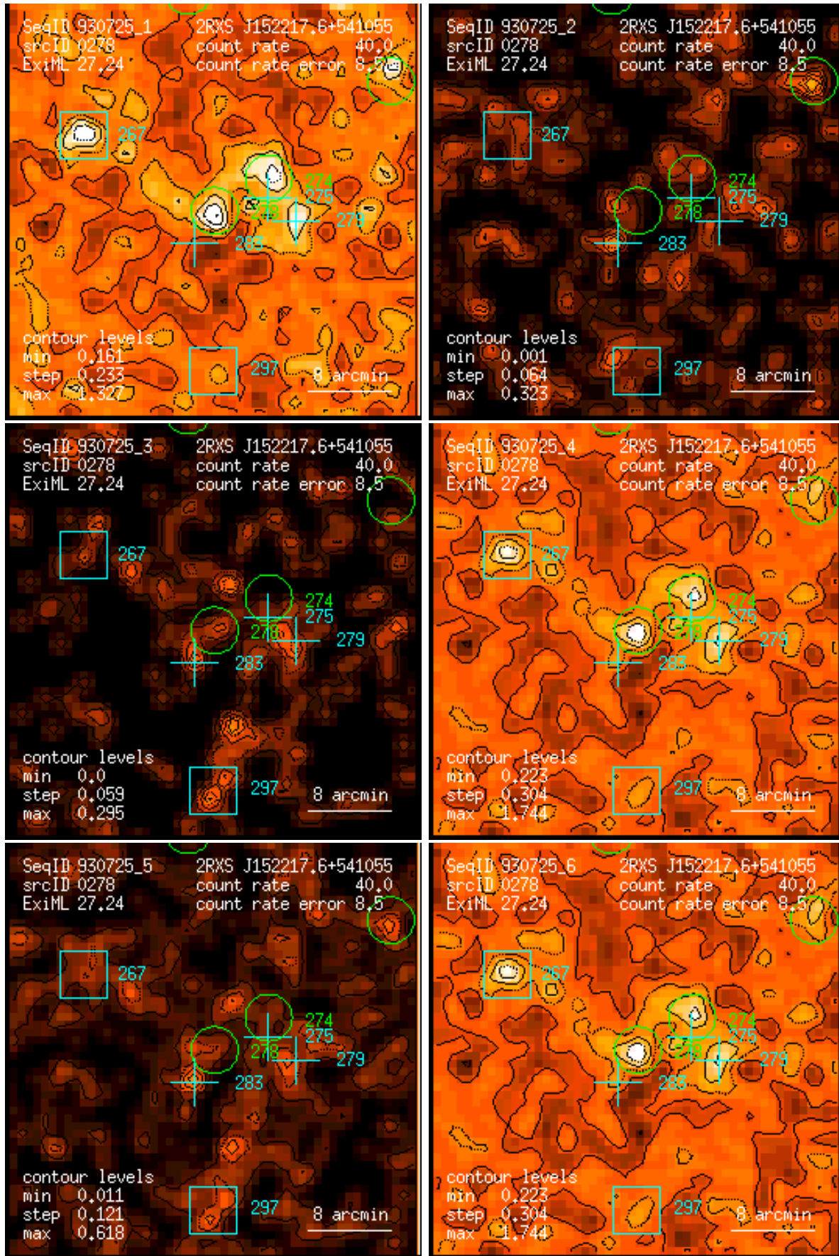
Figure 278: RASS 930725: detection 0278: band rate images, Gaussian filter: (1) PSPC channels 11 – 41, (2) 52 – 90, (3) 91 – 201, (4) 11 – 235, (5) 52 – 201, (6) 11 – 201. Broad band rates in counts/ks. Band rate contour levels in counts/ks/arcmin 2 .
