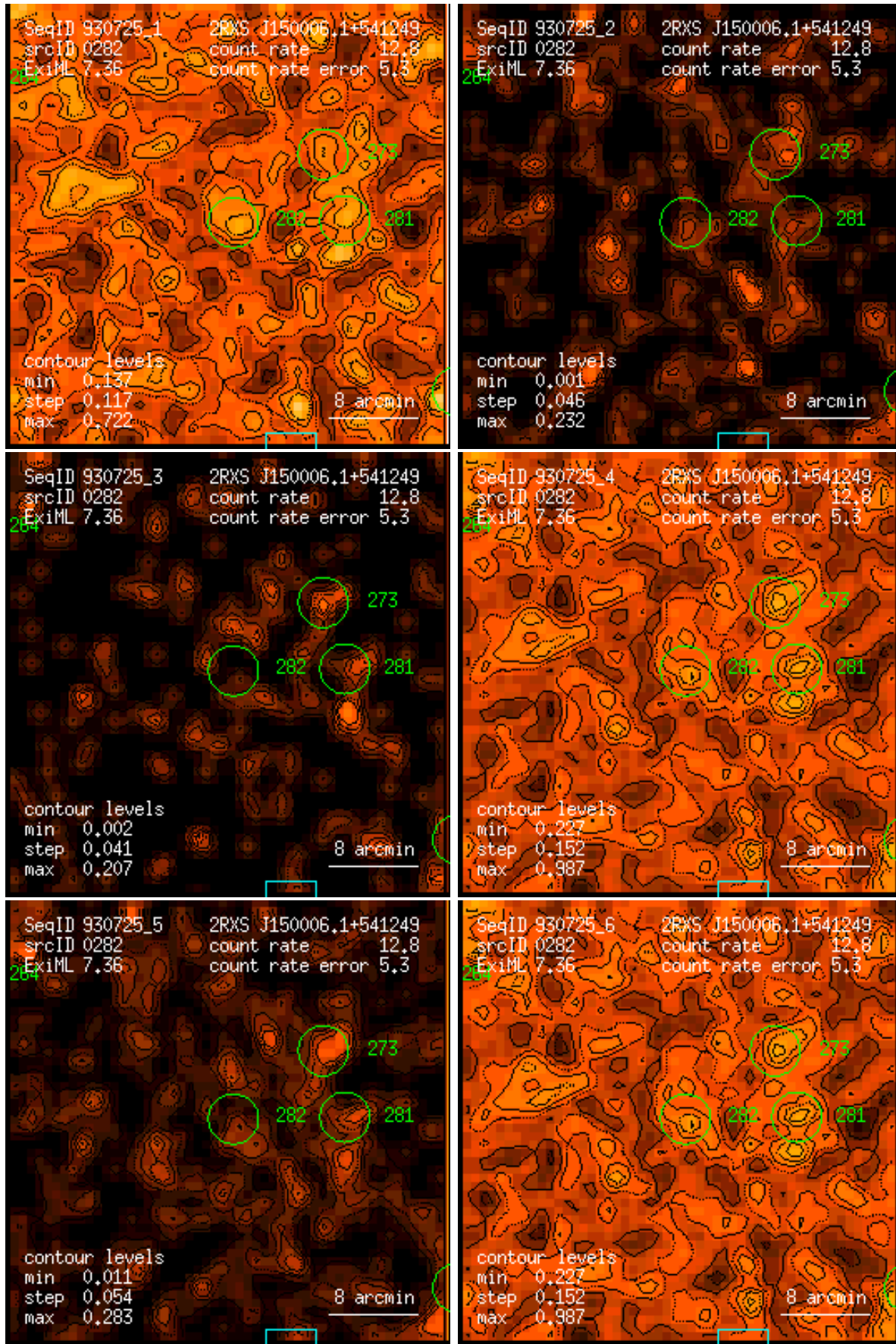
Figure 282: RASS 930725: detection 0282: band rate images, Gaussian filter: (1) PSPC channels 11 – 41, (2) 52 – 90, (3) 91 – 201, (4) 11 – 235, (5) 52 – 201, (6) 11 – 201. Broad band rates in counts/ks. Band rate contour levels in counts/ks/arcmin 2 .
