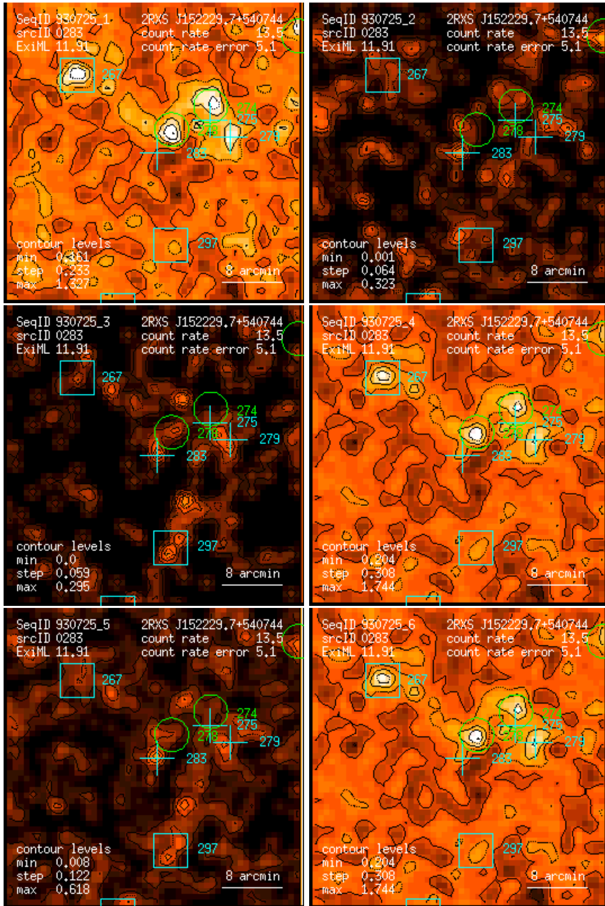
Figure 283: RASS 930725: detection 0283: band rate images, Gaussian filter: (1) PSPC channels 11 – 41, (2) 52 – 90, (3) 91 – 201, (4) 11 – 235, (5) 52 – 201, (6) 11 – 201. Broad band rates in counts/ks. Band rate contour levels in counts/ks/arcmin 2 .
