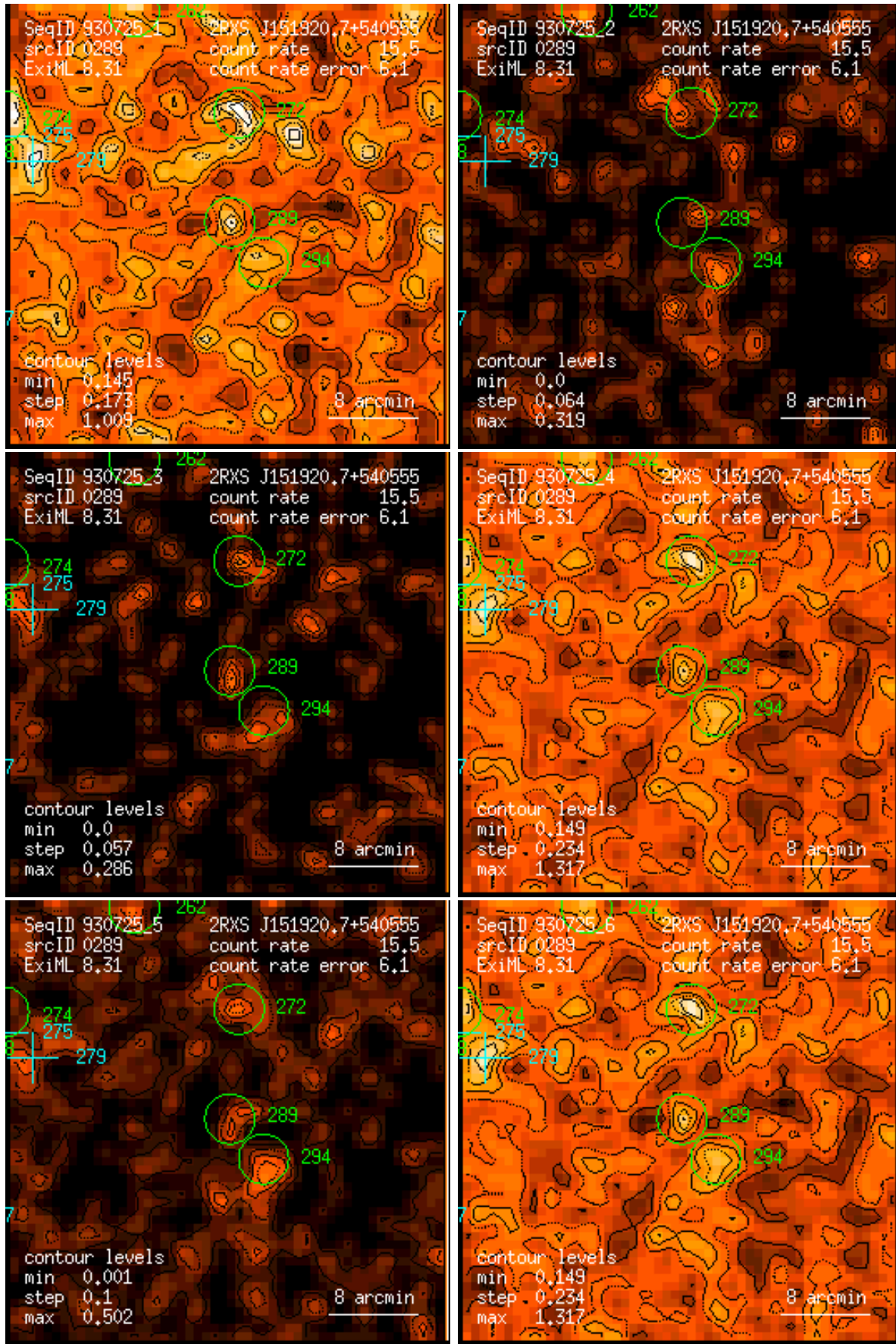
Figure 289: RASS 930725: detection 0289: band rate images, Gaussian filter: (1) PSPC channels 11 – 41, (2) 52 – 90, (3) 91 – 201, (4) 11 – 235, (5) 52 – 201, (6) 11 – 201. Broad band rates in counts/ks. Band rate contour levels in counts/ks/arcmin 2 .
