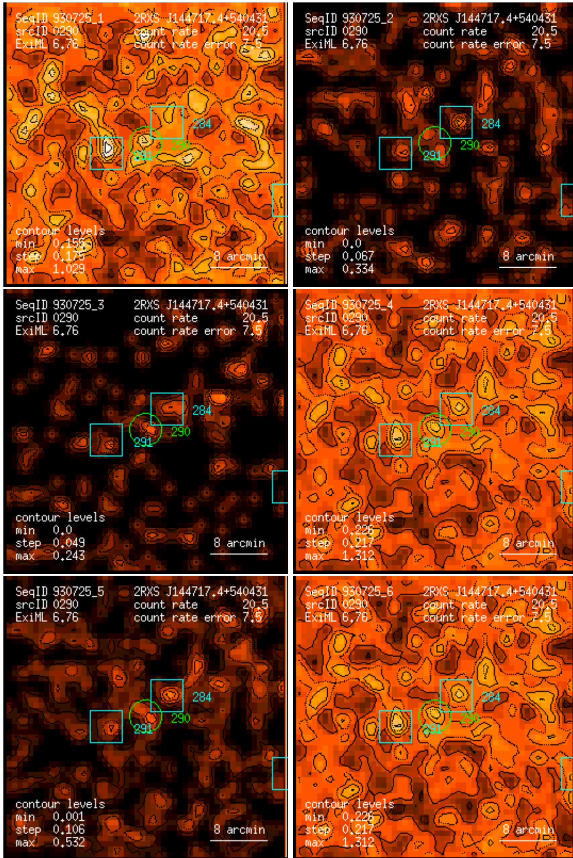
Figure 290: RASS 930725: detection 0290: band rate images, Gaussian filter: (1) PSPC channels 11 – 41, (2) 52 – 90, (3) 91 – 201, (4) 11 – 235, (5) 52 – 201, (6) 11 – 201. Broad band rates in counts/ks. Band rate contour levels in counts/ks/arcmin 2 .
