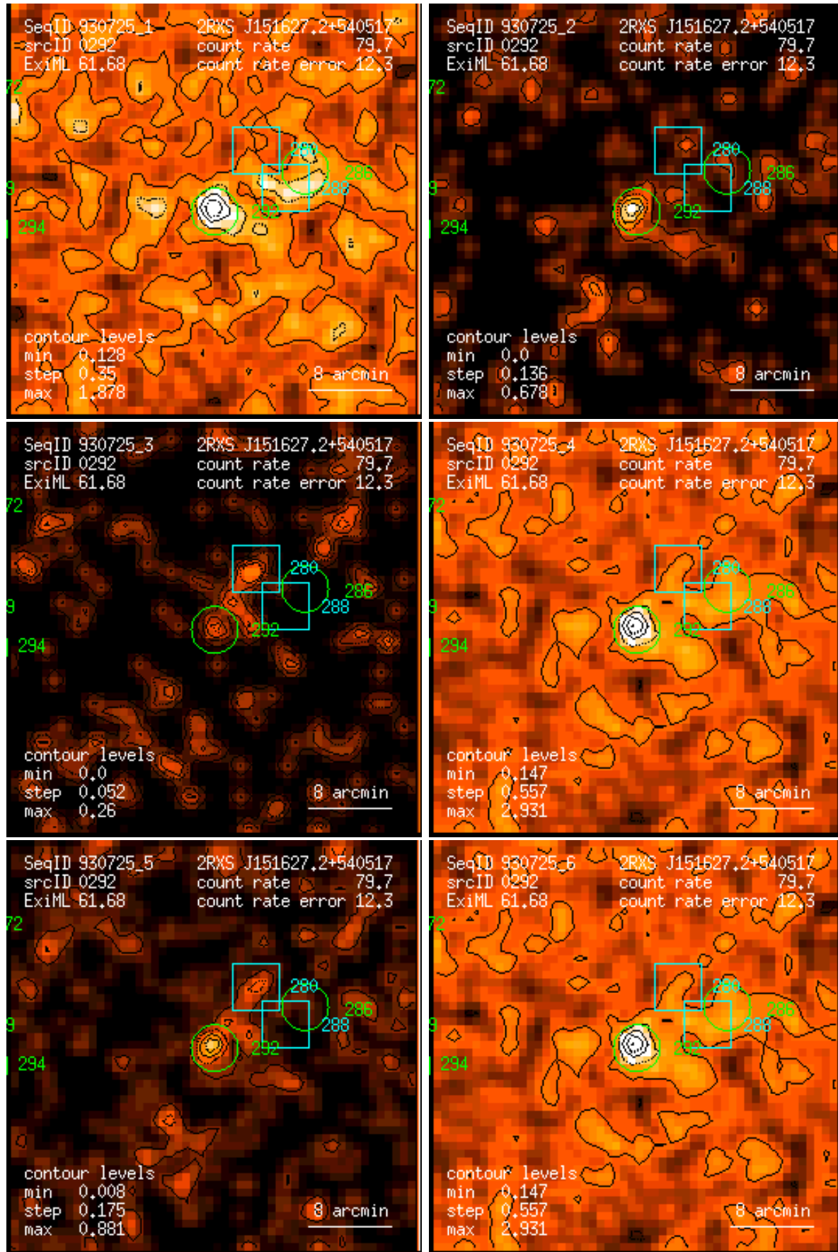
Figure 292: RASS 930725: detection 0292: band rate images, Gaussian filter: (1) PSPC channels 11 – 41, (2) 52 – 90, (3) 91 – 201, (4) 11 – 235, (5) 52 – 201, (6) 11 – 201. Broad band rates in counts/ks. Band rate contour levels in counts/ks/arcmin 2 .
