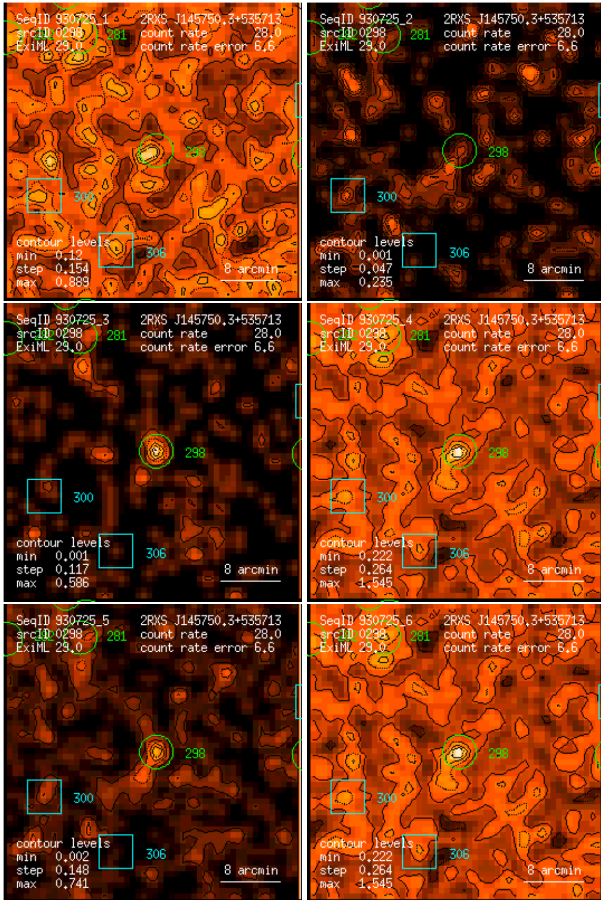
Figure 298: RASS 930725: detection 0298: band rate images, Gaussian filter: (1) PSPC channels 11 – 41, (2) 52 – 90, (3) 91 – 201, (4) 11 – 235, (5) 52 – 201, (6) 11 – 201. Broad band rates in counts/ks. Band rate contour levels in counts/ks/arcmin 2 .
