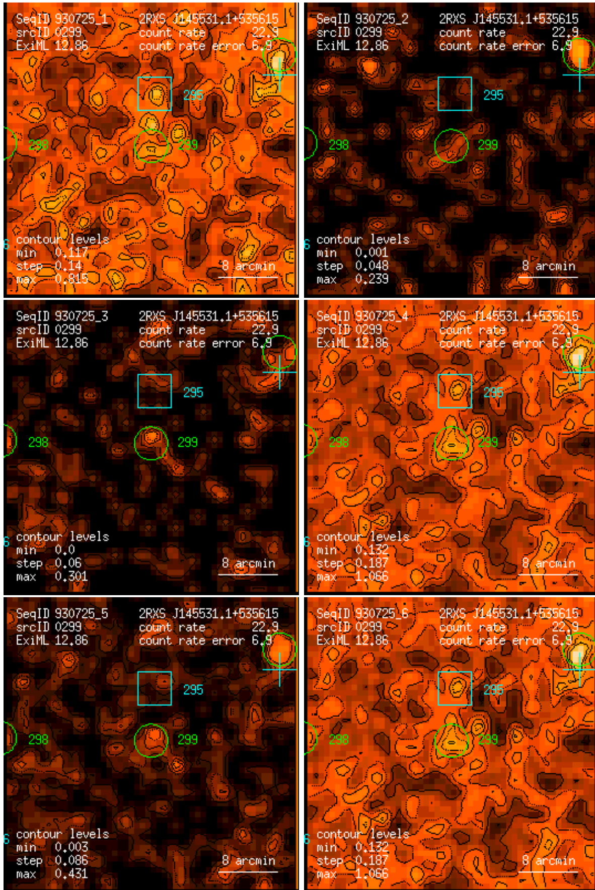
Figure 299: RASS 930725: detection 0299: band rate images, Gaussian filter: (1) PSPC channels 11 – 41, (2) 52 – 90, (3) 91 – 201, (4) 11 – 235, (5) 52 – 201, (6) 11 – 201. Broad band rates in counts/ks. Band rate contour levels in counts/ks/arcmin 2 .
