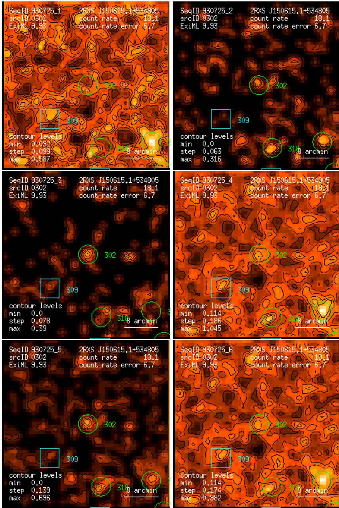
Figure 302: RASS 930725: detection 0302: band rate images, Gaussian filter: (1) PSPC channels 11 – 41, (2) 52 – 90, (3) 91 – 201, (4) 11 – 235, (5) 52 – 201, (6) 11 – 201. Broad band rates in counts/ks. Band rate contour levels in counts/ks/arcmin 2 .
