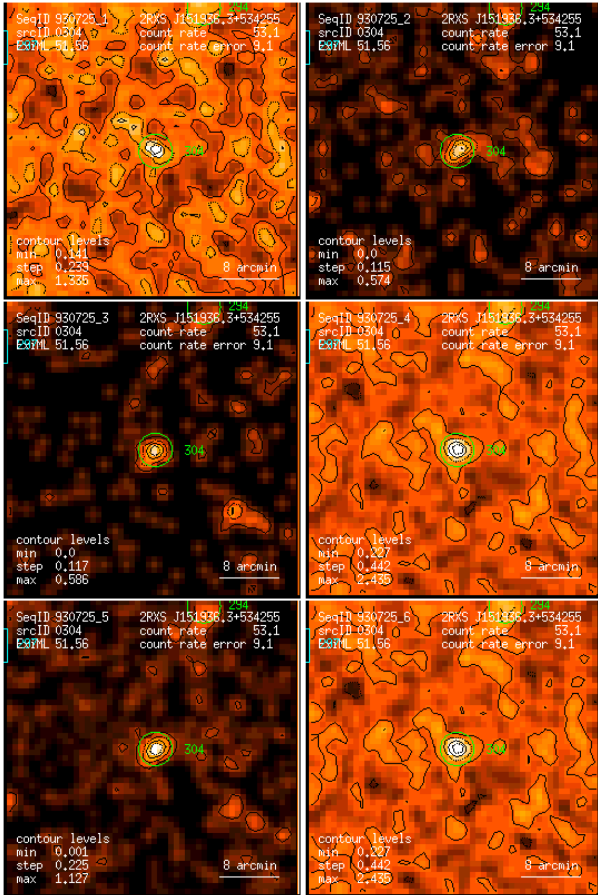
Figure 304: RASS 930725: detection 0304: band rate images, Gaussian filter: (1) PSPC channels 11 – 41, (2) 52 – 90, (3) 91 – 201, (4) 11 – 235, (5) 52 – 201, (6) 11 – 201. Broad band rates in counts/ks. Band rate contour levels in counts/ks/arcmin 2 .
