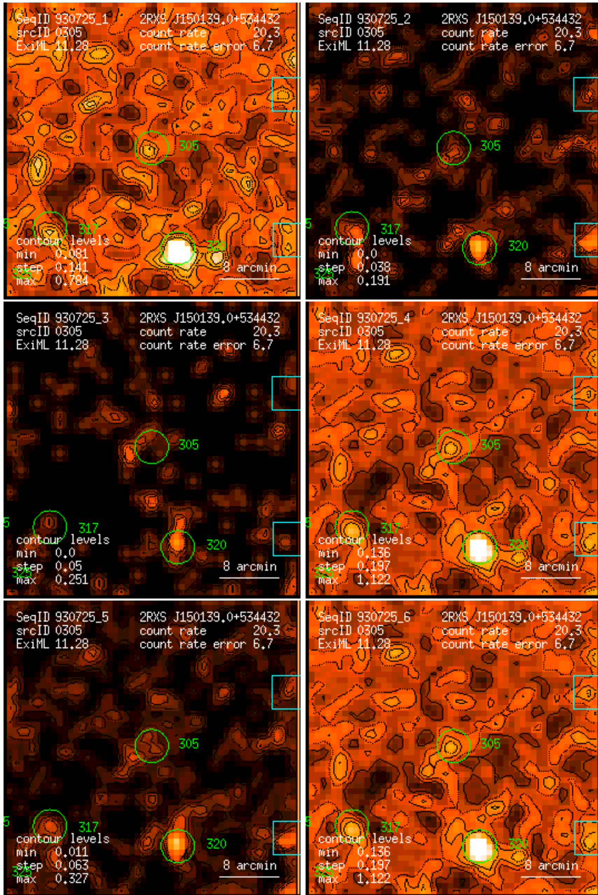
Figure 305: RASS 930725: detection 0305: band rate images, Gaussian filter: (1) PSPC channels 11 – 41, (2) 52 – 90, (3) 91 – 201, (4) 11 – 235, (5) 52 – 201, (6) 11 – 201. Broad band rates in counts/ks. Band rate contour levels in counts/ks/arcmin 2 .
