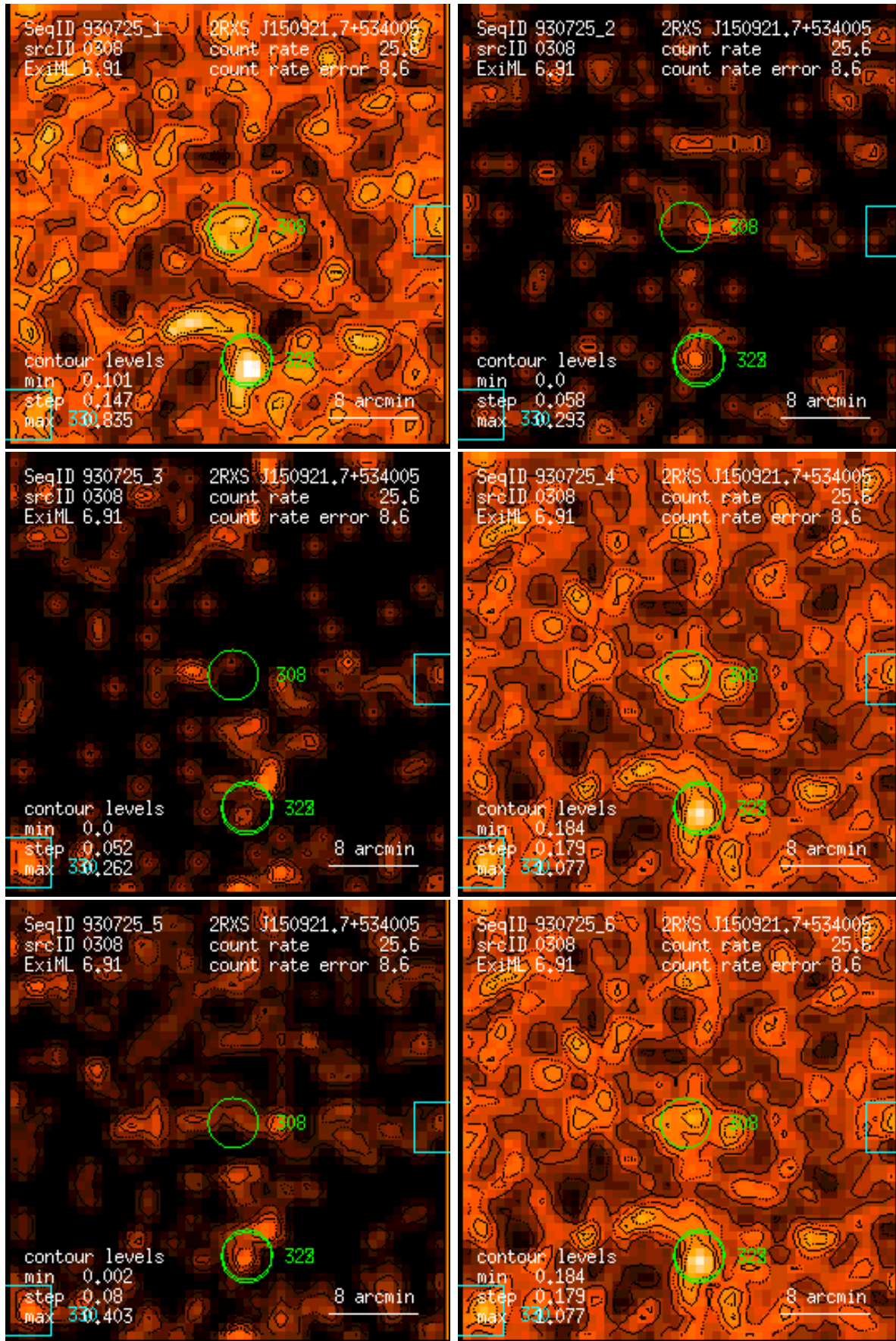
Figure 308: RASS 930725: detection 0308: band rate images, Gaussian filter: (1) PSPC channels 11 – 41, (2) 52 – 90, (3) 91 – 201, (4) 11 – 235, (5) 52 – 201, (6) 11 – 201. Broad band rates in counts/ks. Band rate contour levels in counts/ks/arcmin 2 .
