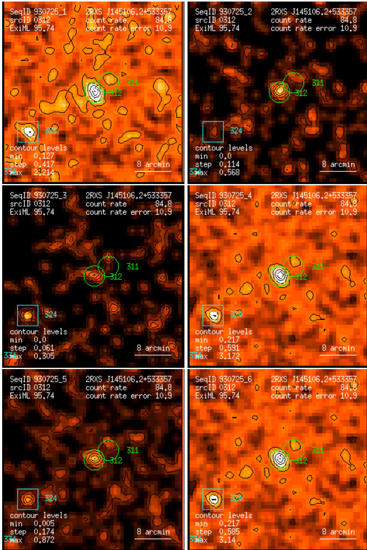
Figure 312: RASS 930725: detection 0312: band rate images, Gaussian filter: (1) PSPC channels 11 – 41, (2) 52 – 90, (3) 91 – 201, (4) 11 – 235, (5) 52 – 201, (6) 11 – 201. Broad band rates in counts/ks. Band rate contour levels in counts/ks/arcmin 2 .
