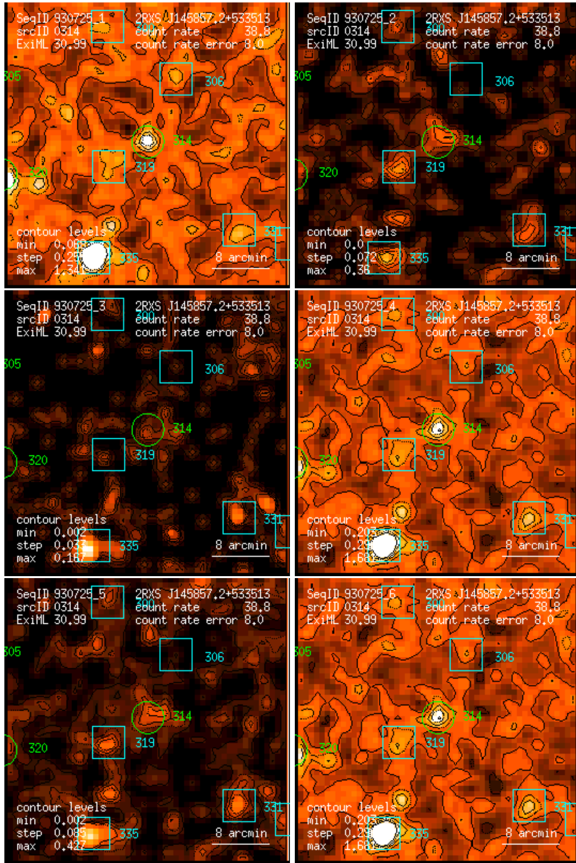
Figure 314: RASS 930725: detection 0314: band rate images, Gaussian filter: (1) PSPC channels 11 – 41, (2) 52 – 90, (3) 91 – 201, (4) 11 – 235, (5) 52 – 201, (6) 11 – 201. Broad band rates in counts/ks. Band rate contour levels in counts/ks/arcmin 2 .
