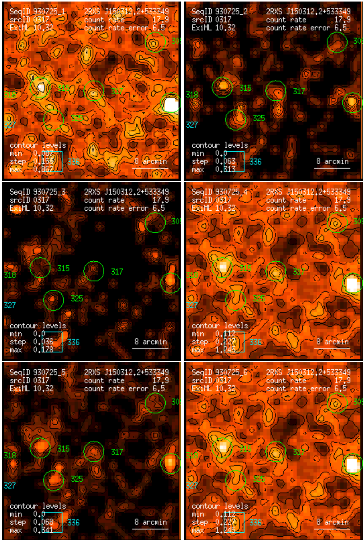
Figure 317: RASS 930725: detection 0317: band rate images, Gaussian filter: (1) PSPC channels 11 – 41, (2) 52 – 90, (3) 91 – 201, (4) 11 – 235, (5) 52 – 201, (6) 11 – 201. Broad band rates in counts/ks. Band rate contour levels in counts/ks/arcmin 2 .
