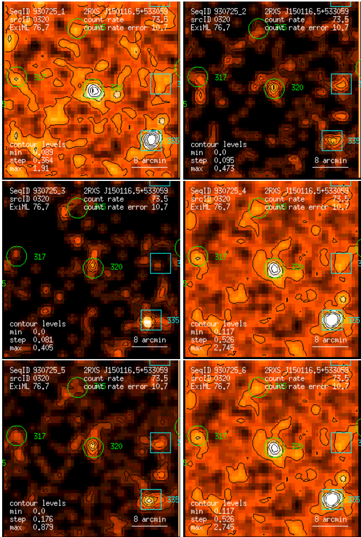
Figure 320: RASS 930725: detection 0320: band rate images, Gaussian filter: (1) PSPC channels 11 – 41, (2) 52 – 90, (3) 91 – 201, (4) 11 – 235, (5) 52 – 201, (6) 11 – 201. Broad band rates in counts/ks. Band rate contour levels in counts/ks/arcmin 2 .
