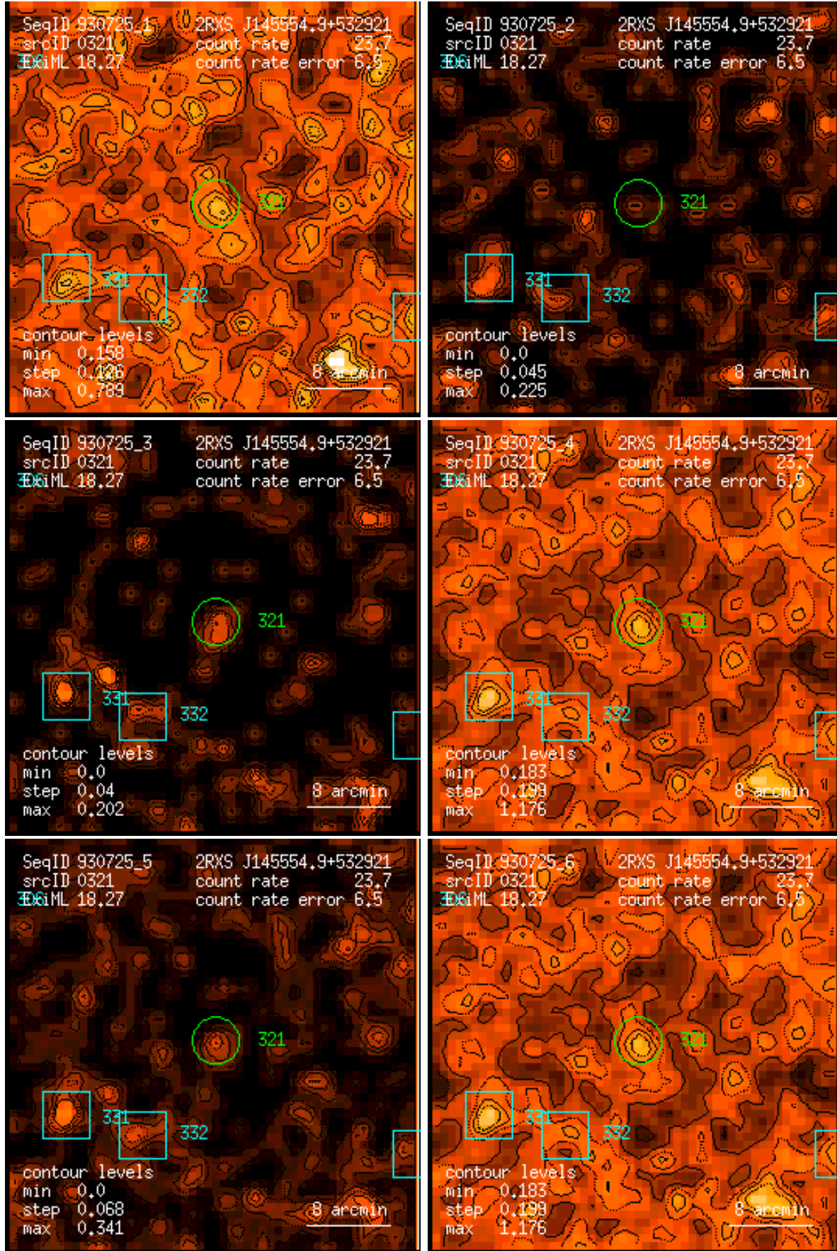
Figure 321: RASS 930725: detection 0321: band rate images, Gaussian filter: (1) PSPC channels 11 – 41, (2) 52 – 90, (3) 91 – 201, (4) 11 – 235, (5) 52 – 201, (6) 11 – 201. Broad band rates in counts/ks. Band rate contour levels in counts/ks/arcmin 2 .
