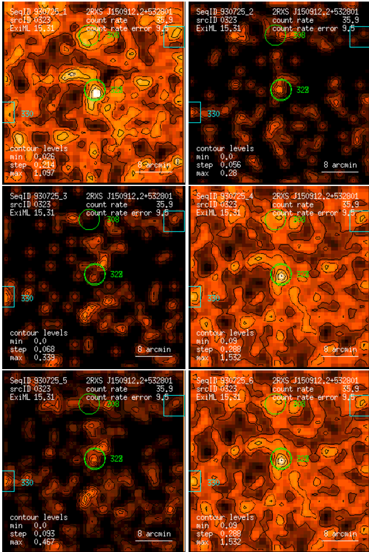
Figure 323: RASS 930725: detection 0323: band rate images, Gaussian filter: (1) PSPC channels 11 – 41, (2) 52 – 90, (3) 91 – 201, (4) 11 – 235, (5) 52 – 201, (6) 11 – 201. Broad band rates in counts/ks. Band rate contour levels in counts/ks/arcmin 2 .
