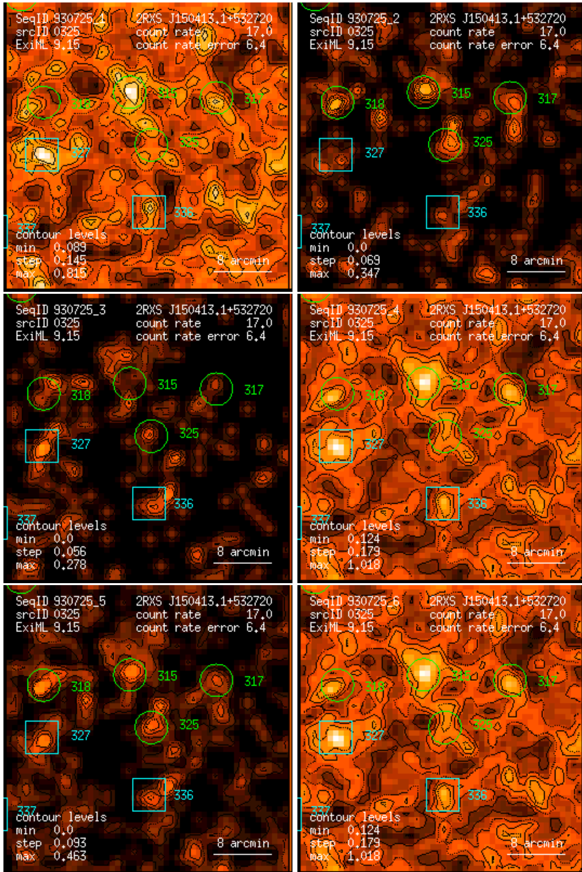
Figure 325: RASS 930725: detection 0325: band rate images, Gaussian filter: (1) PSPC channels 11 – 41, (2) 52 – 90, (3) 91 – 201, (4) 11 – 235, (5) 52 – 201, (6) 11 – 201. Broad band rates in counts/ks. Band rate contour levels in counts/ks/arcmin 2 .
