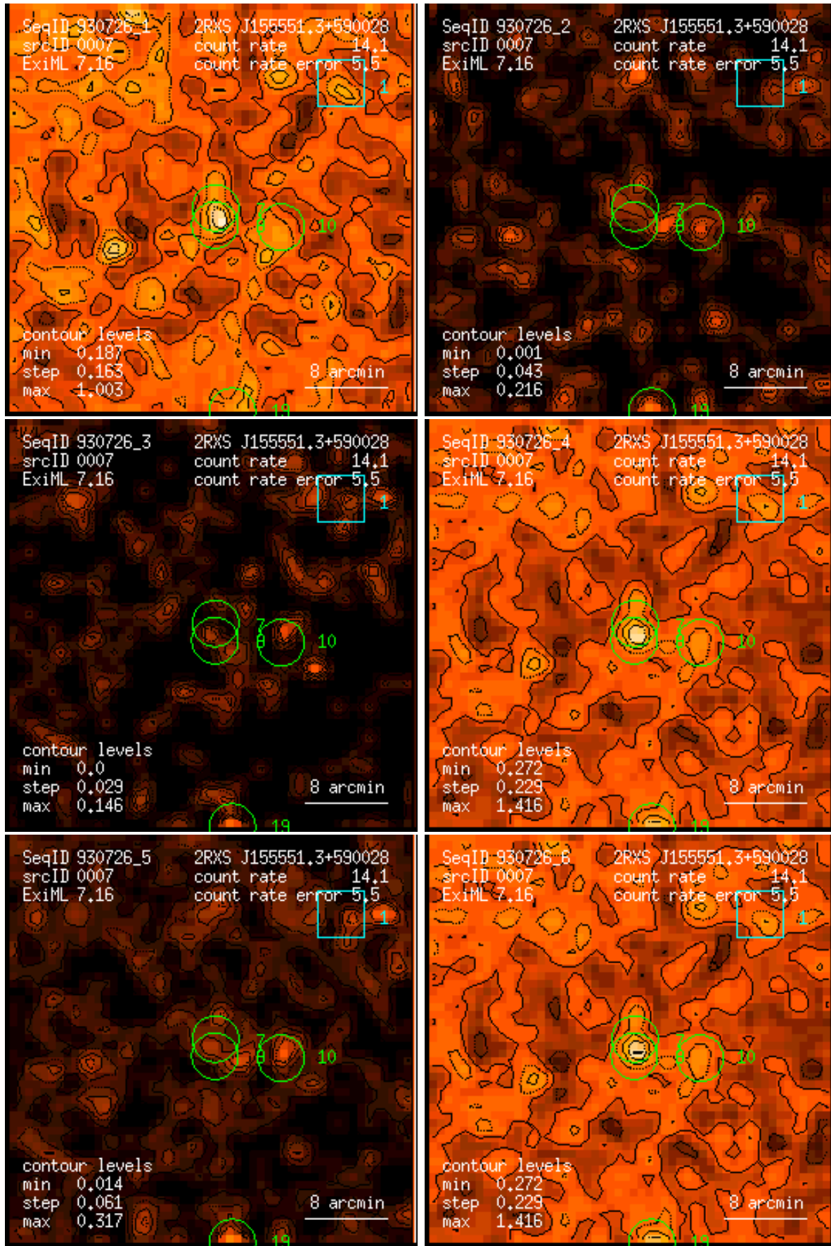
Figure 7: RASS 930726: detection 0007: band rate images, Gaussian filter: (1) PSPC channels 11 – 41, (2) 52 – 90, (3) 91 – 201, (4) 11 – 235, (5) 52 – 201, (6) 11 – 201. Broad band rates in counts/ks. Band rate contour levels in counts/ks/arcmin 2 .
