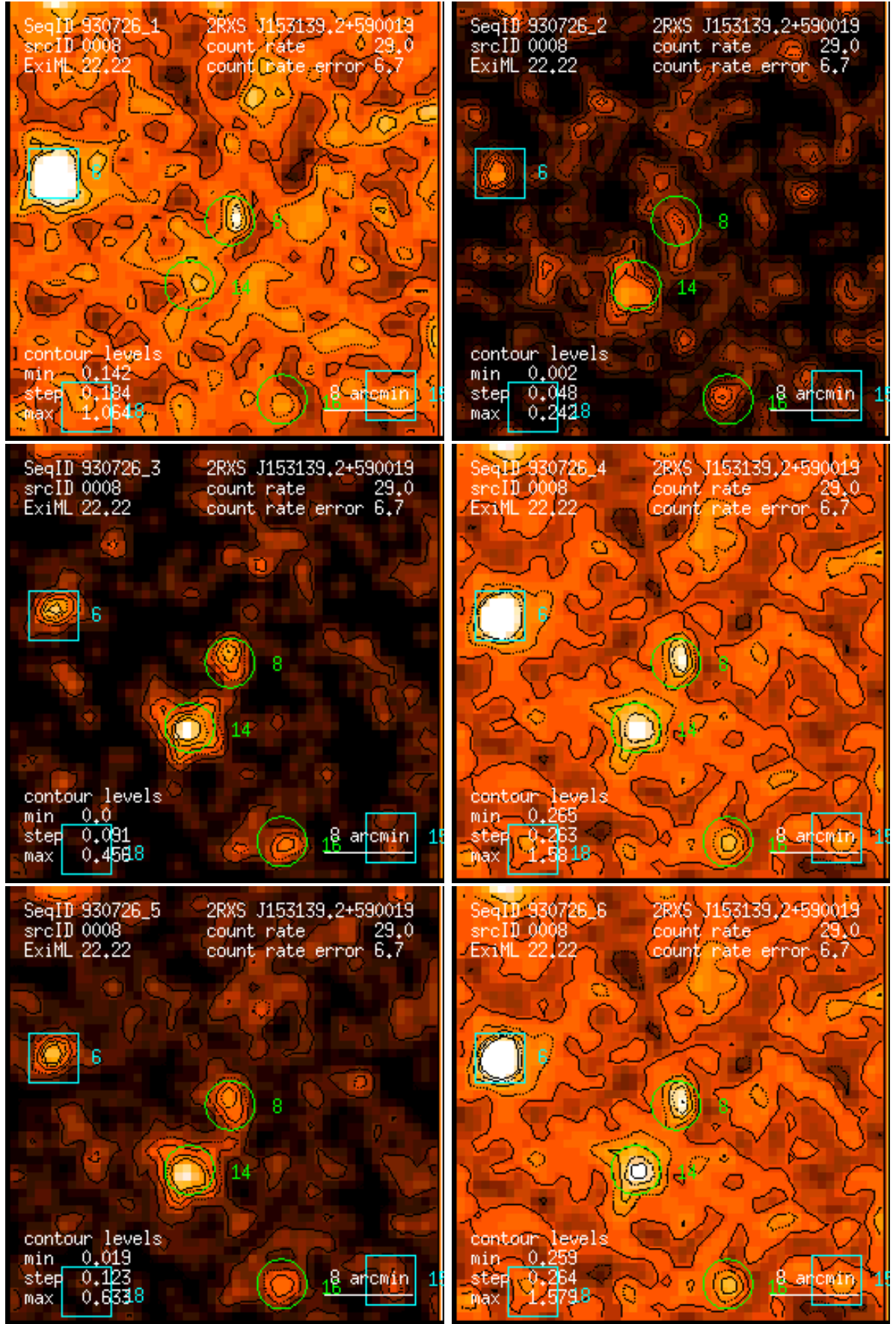
Figure 8: RASS 930726: detection 0008: band rate images, Gaussian filter: (1) PSPC channels 11 – 41, (2) 52 – 90, (3) 91 – 201, (4) 11 – 235, (5) 52 – 201, (6) 11 – 201. Broad band rates in counts/ks. Band rate contour levels in counts/ks/arcmin 2 .
