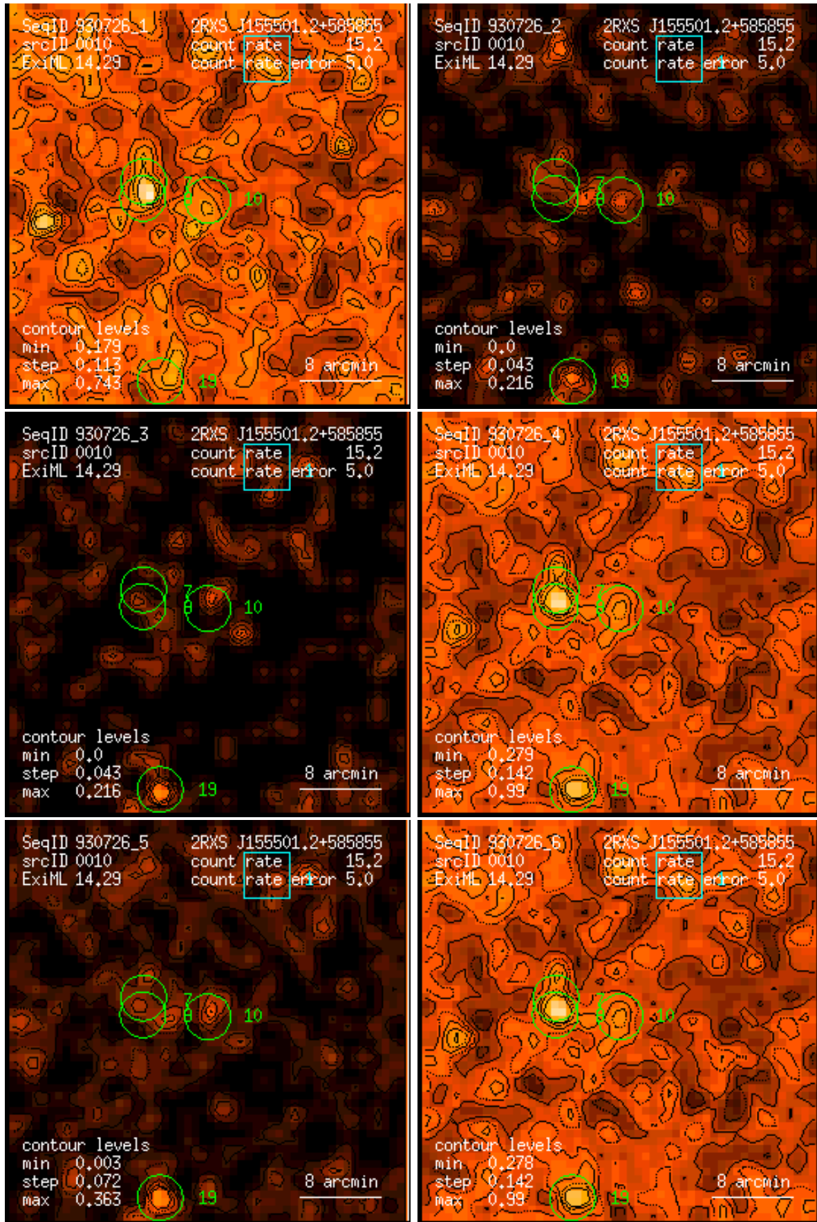
Figure 10: RASS 930726: detection 0010: band rate images, Gaussian filter: (1) PSPC channels 11 – 41, (2) 52 – 90, (3) 91 – 201, (4) 11 – 235, (5) 52 – 201, (6) 11 – 201. Broad band rates in counts/ks. Band rate contour levels in counts/ks/arcmin 2 .
