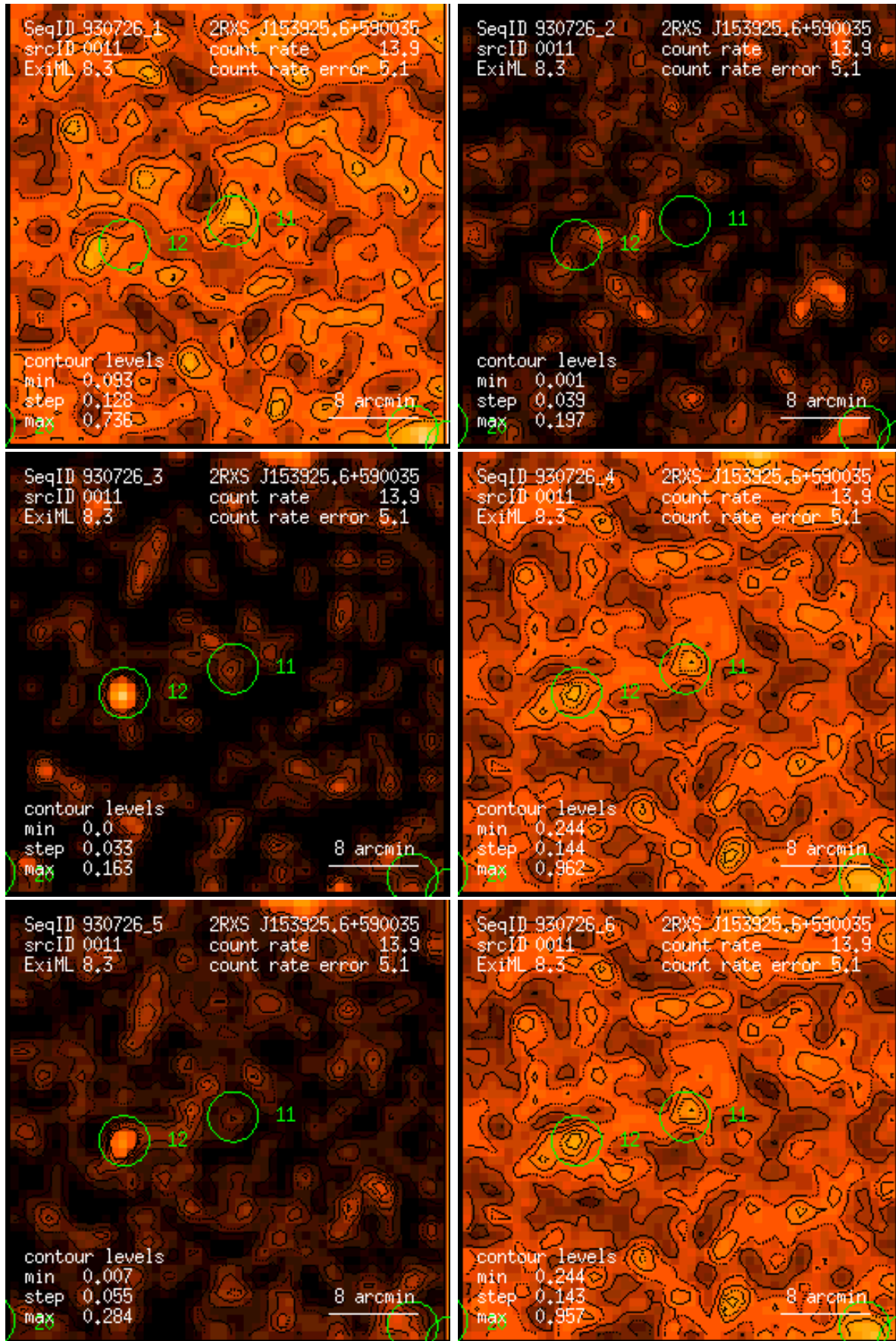
Figure 11: RASS 930726: detection 0011: band rate images, Gaussian filter: (1) PSPC channels 11 – 41, (2) 52 – 90, (3) 91 – 201, (4) 11 – 235, (5) 52 – 201, (6) 11 – 201. Broad band rates in counts/ks. Band rate contour levels in counts/ks/arcmin 2 .
