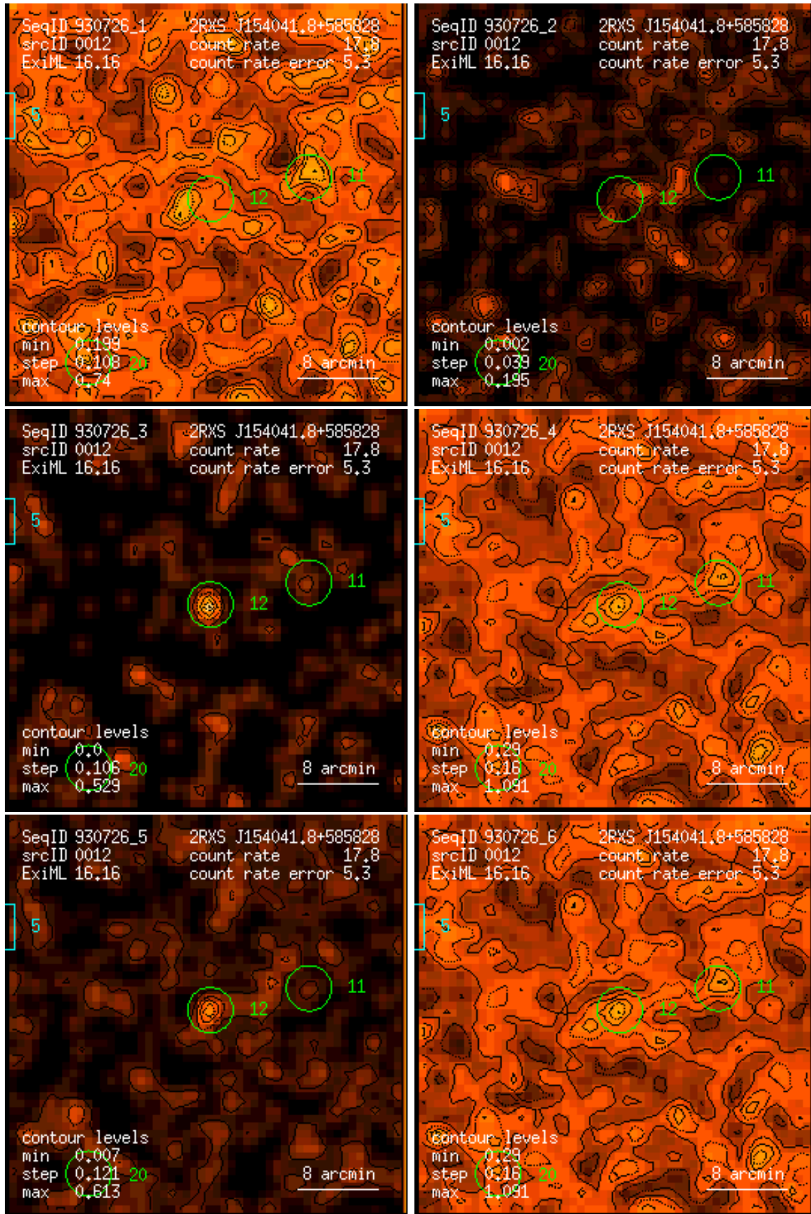
Figure 12: RASS 930726: detection 0012: band rate images, Gaussian filter: (1) PSPC channels 11 – 41, (2) 52 – 90, (3) 91 – 201, (4) 11 – 235, (5) 52 – 201, (6) 11 – 201. Broad band rates in counts/ks. Band rate contour levels in counts/ks/arcmin 2 .
