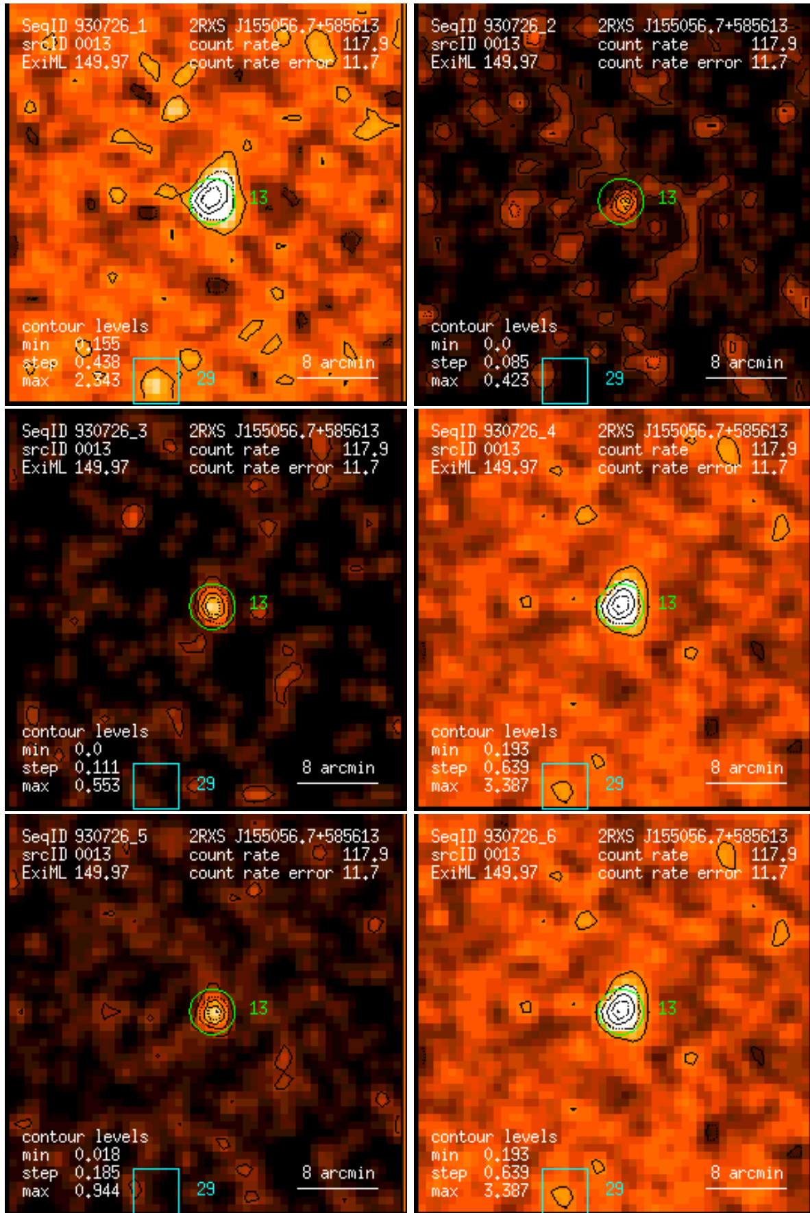
Figure 13: RASS 930726: detection 0013: band rate images, Gaussian filter: (1) PSPC channels 11 – 41, (2) 52 – 90, (3) 91 – 201, (4) 11 – 235, (5) 52 – 201, (6) 11 – 201. Broad band rates in counts/ks. Band rate contour levels in counts/ks/arcmin 2 .
