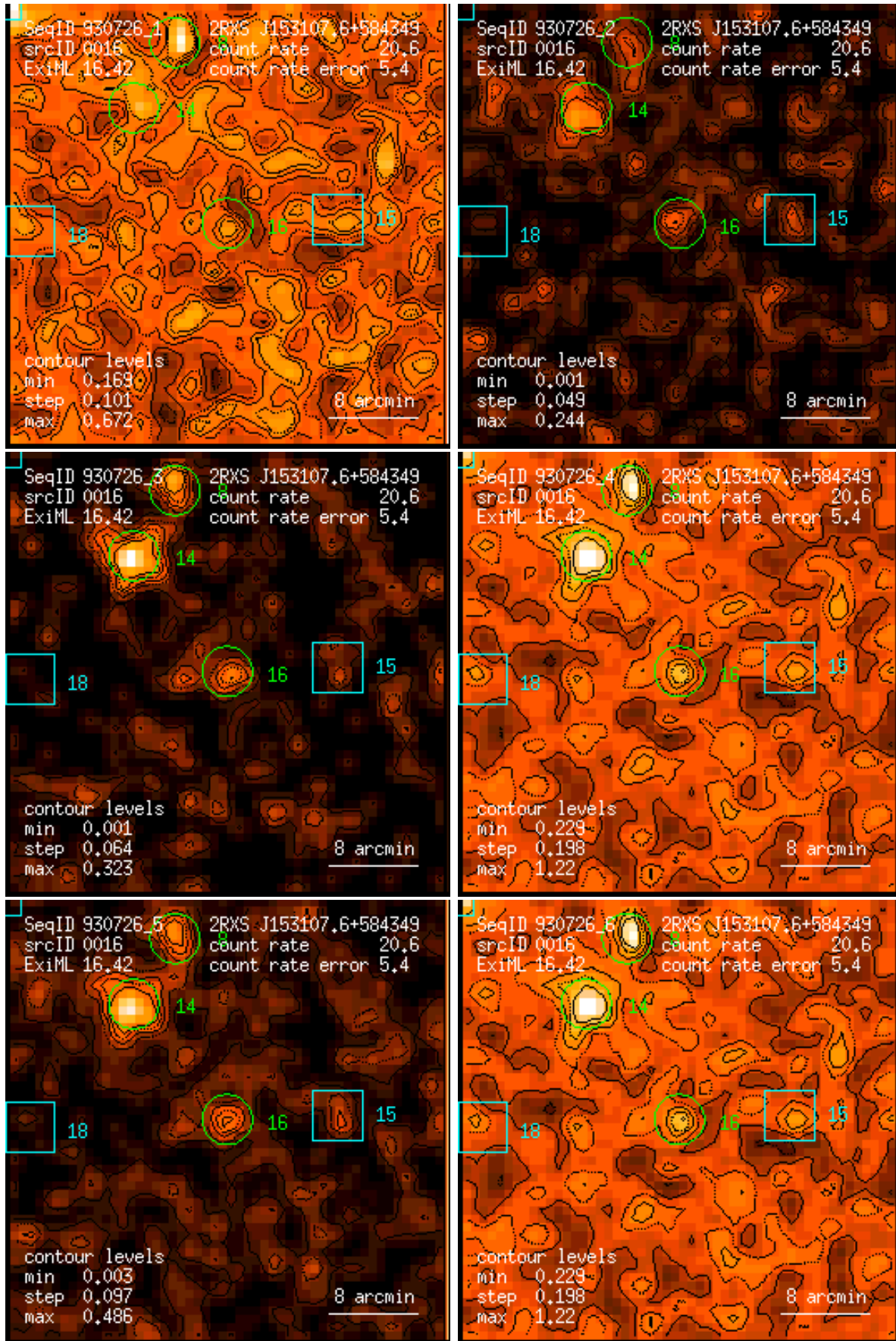
Figure 16: RASS 930726: detection 0016: band rate images, Gaussian filter: (1) PSPC channels 11 – 41, (2) 52 – 90, (3) 91 – 201, (4) 11 – 235, (5) 52 – 201, (6) 11 – 201. Broad band rates in counts/ks. Band rate contour levels in counts/ks/arcmin 2 .
